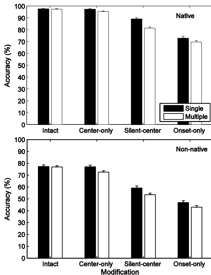
Fig. 3. Accuracy of identification of single- and multiple-speaker tones by native listeners (Lee, Tao, & Bond, 2009) and non-native listeners (Lee, Tao, & Bond, 2010a). Error bar indicates standard error.
