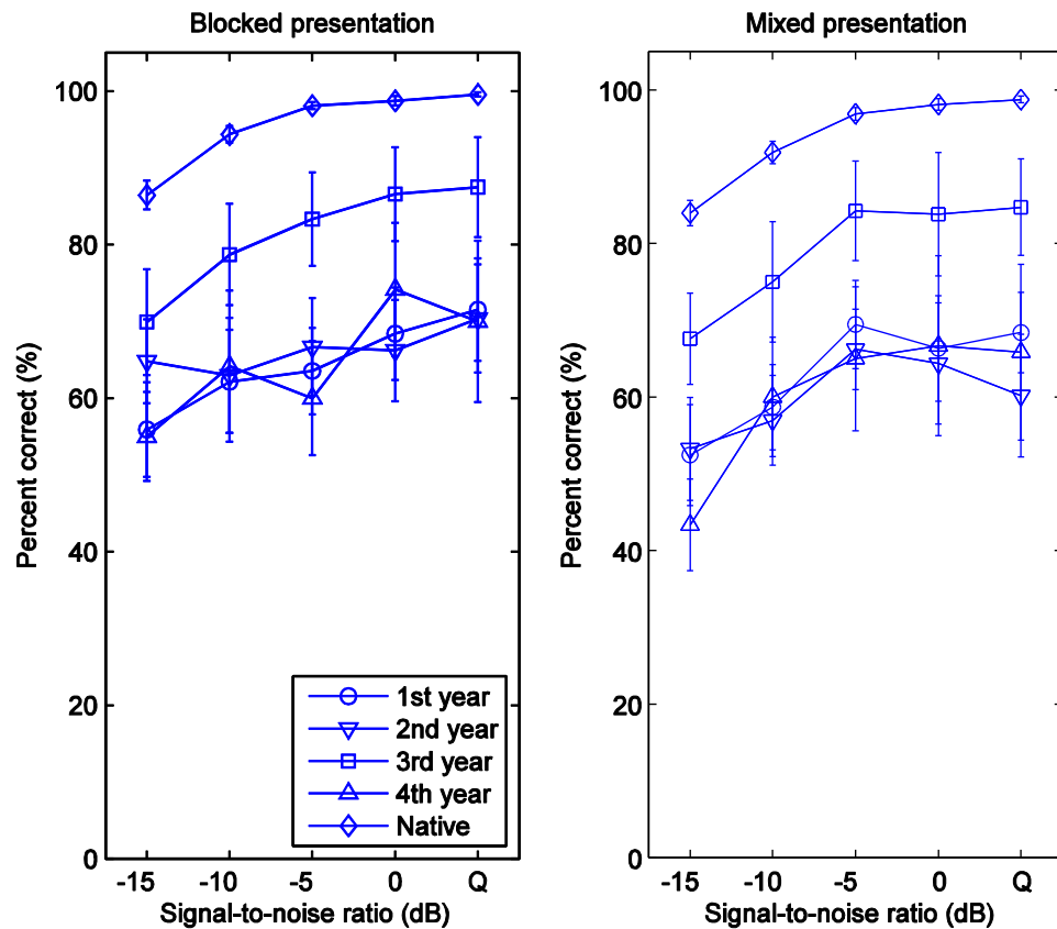
Fig. 4. Accuracy of Mandarin tone identification as a function of speaker variability (blocked/mixed presentation), noise level (quiet to -15 dB SNR), and listener background (native and 1-4 years of instruction) in Lee, Tao, and Bond (2010b), reproduced with permission from Elsevier. Error bar indicates standard error.
