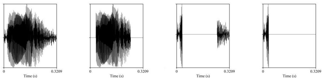
Fig. 2. From left: intact, center-only, silent-center, and onset-only stimuli.
