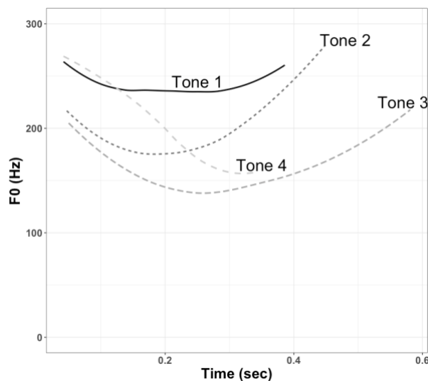
Fig. 1. F0 contours of the four Mandarin tones.
