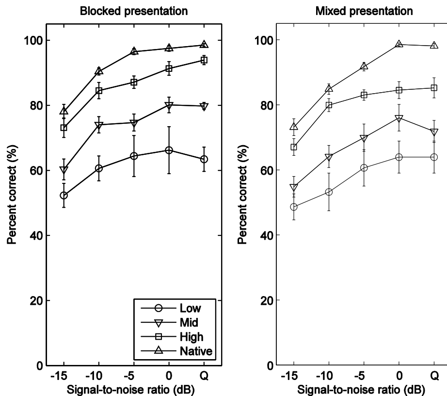
Fig. 5. Accuracy of Mandarin tone identification as a function of speaker variability (blocked/mixed presentation), noise level (quiet to -15 dB SNR), and listener background (native and level of proficiency) in Lee, Tao, and Bond (2013), reproduced with permission from Taylor & Francis Ltd. Error bar indicates standard error.
