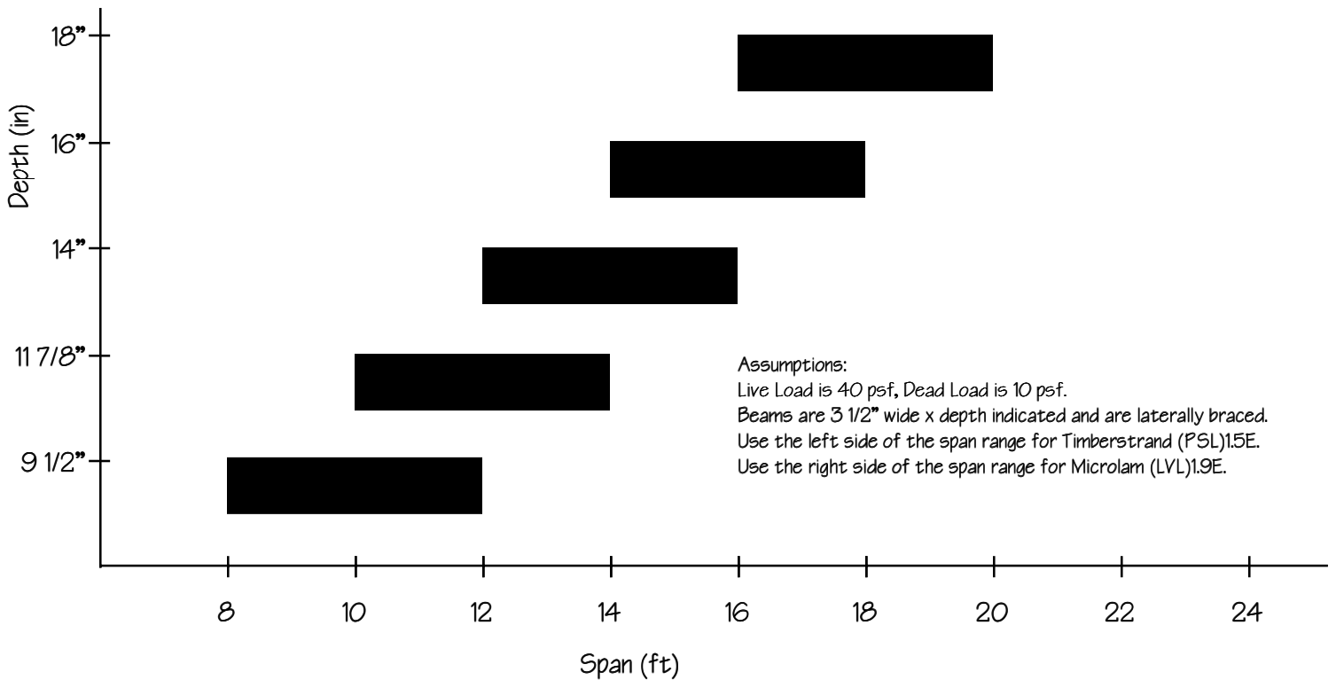
Approximate Span Table for Timberstrand and Microlam Engineered Wood Beams
