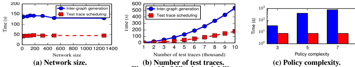
Figure 12: Mikado scalability.
