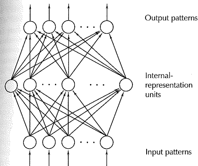
Figure 8.3: A multilayer network in which input patterns are recoded by internal representation units.
