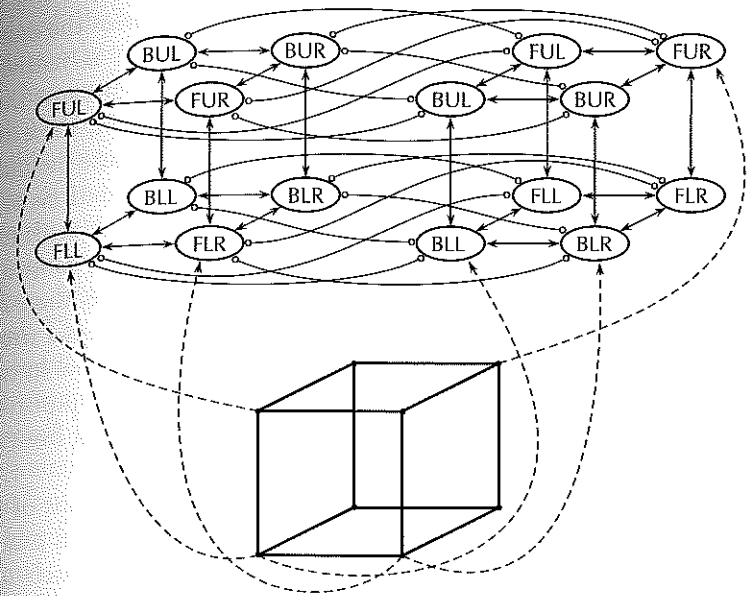
Figure 8.2: A simple network representing some constraints involved in perceiving a Necker cube. The ovals are the units in the network; connections with arrow-heads are positive (excitatory), while those with circle-heads are negative (inhibitory); the dotted lines represent input stimuli from the perceived cube.
