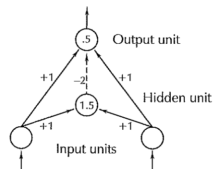
Figure 8.4: A simple XOR network with one hidden unit.
