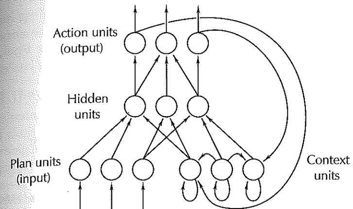
Figure 8.5: A recurrent network of the type developed by Jordan (1986) for learning to perform sequential operations.
