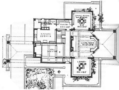
FLW, "Home for a Prairie Town," 1900
