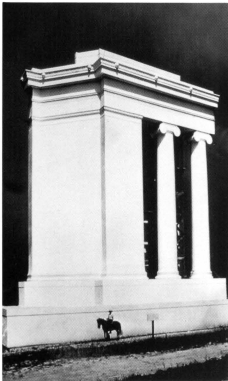
Mellon Institute's focus on experimentation was applied in the design of its own new building. In 1931, a full-scale model of a corner pier and two columns were erected in Fox Chapel, and studied for 19 months.
