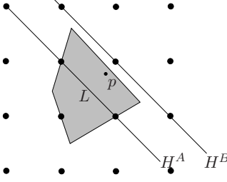
Figure 12: Illustration for the statement of Lemma 5.13 with m = 2 . Polytope Q is shaded and polytope L is a segment.
