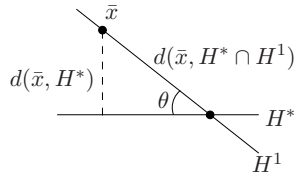
Figure 6: Illustration for the proof of Observation 5.3.
