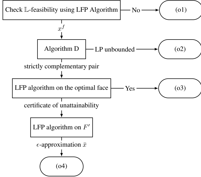
Figure 1: Schematic description of the \mathbb{L} -linear program solver
