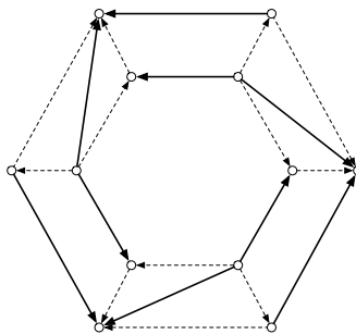
Figure 1: The solid arcs form an inclusionwise minimal 2-dijoin that cannot be decomposed into two dijoints [19], nor is it a 2-arc-connected flip.
