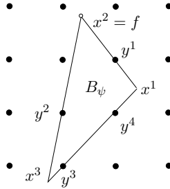
Figure 9: Illustration for Theorem 4.9.
