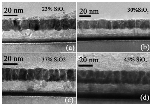
FIG. 1. Cross section TEM images of 16 nm composite FePt-SiOx thin films deposited on MgO/Ta underlayers at 410 °C with different oxide volume fractions in the film.
