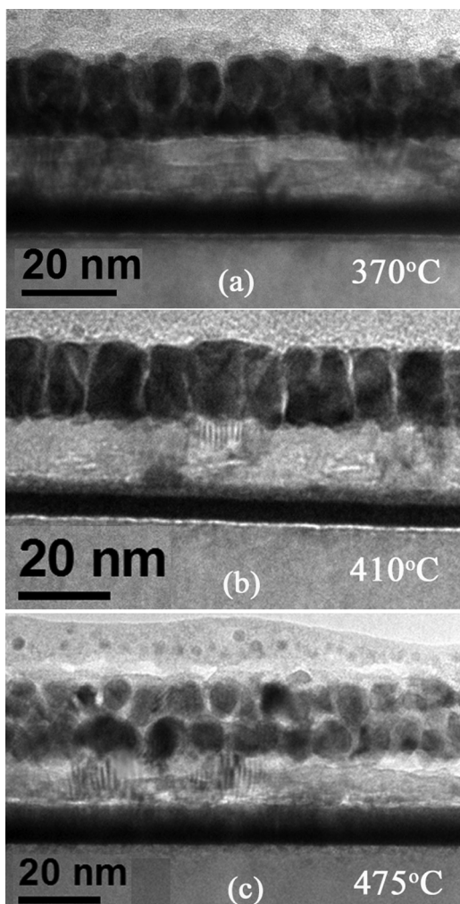
FIG. 2. Cross section TEM images of 16 nm composite FePt-37%SiOx thin films deposited on MgO/Ta underlayers at different substrate temperatures.
