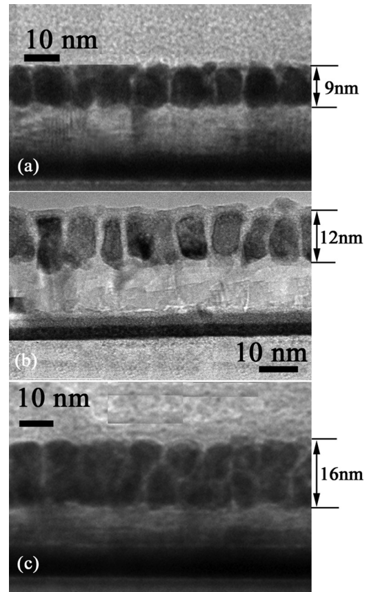
FIG. 3. Cross section TEM images of composite FePt-45%SiOx thin films deposited on MgO/Ta underlayers at 410 °C with different thicknesses of FePt layer.
