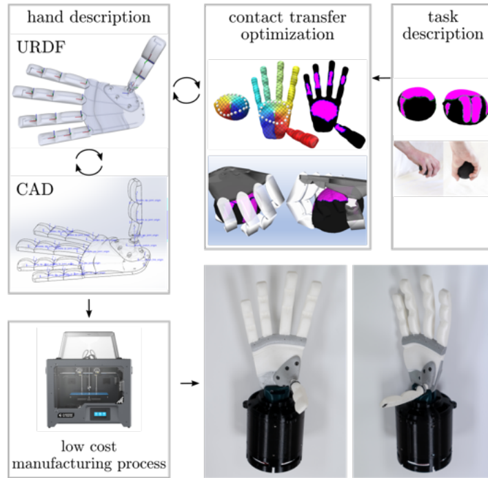
Figure 8.1: Iterative hand design prototyping framework enabled by contact area transfer and grasp computation
