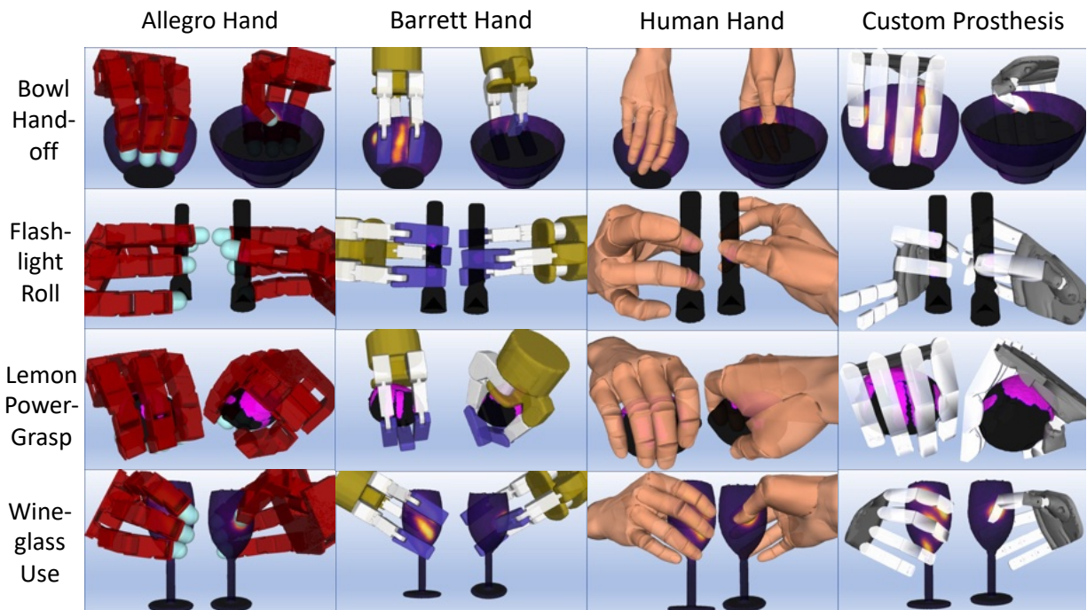
Figure 5.5: Grasps synthesized as a result of our transfer procedure across a variety of kinematically diverse robotic manipulators, objects, and grasps.
