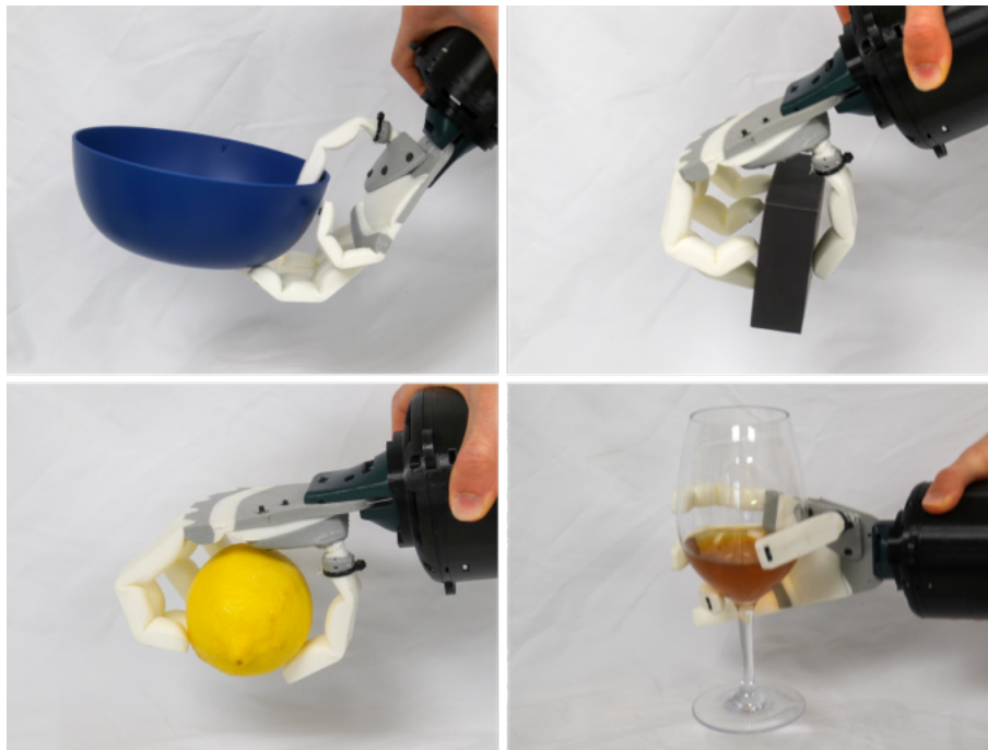
Figure 8.3: Based on the results in the design study shown in Figure 8.2 , candidate (d) is selected for fabrication. All grasps are successfully completed in a pick and place setup using key-framed open-loop poses that match the results obtained in our simulation.
