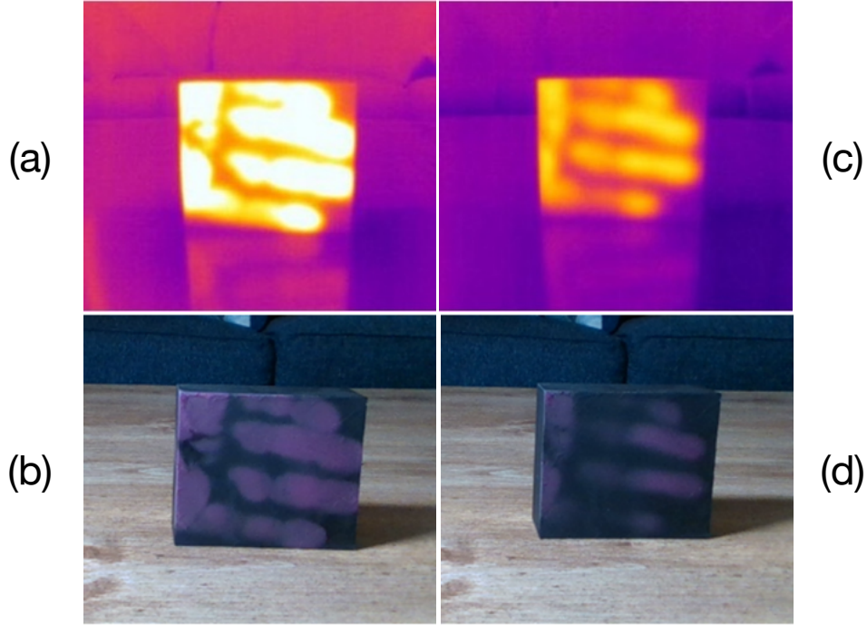
Figure 9.2: Comparison of our (bottom) thermochromic RGB imaging procedure with top a Flir A65 thermal camera at full signal strength (a, b) and after heat dissipation (c, d).
