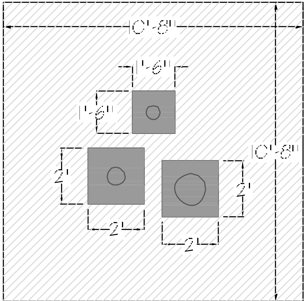
Elevation View
