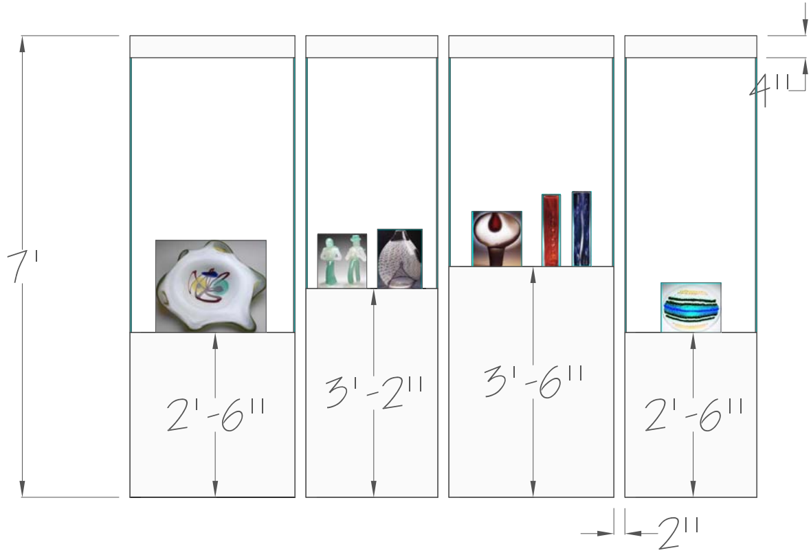
○ Elevation View
