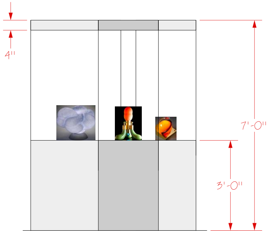
2 Elevation View
