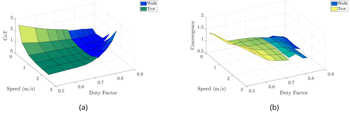
Figure 5.3: The walking and trotting gaits transition quite smoothly between their natural duty factor regimes. Our results indicate the combination of duty factor and speed is a strong predictor of a gait’s energy efficiency, while convergence is primarily correlated with duty factor. Note there are 4 absent data points at the combination of the 2 highest speeds and 2 highest duty factors because the algorithm failed to converge to a solution.
