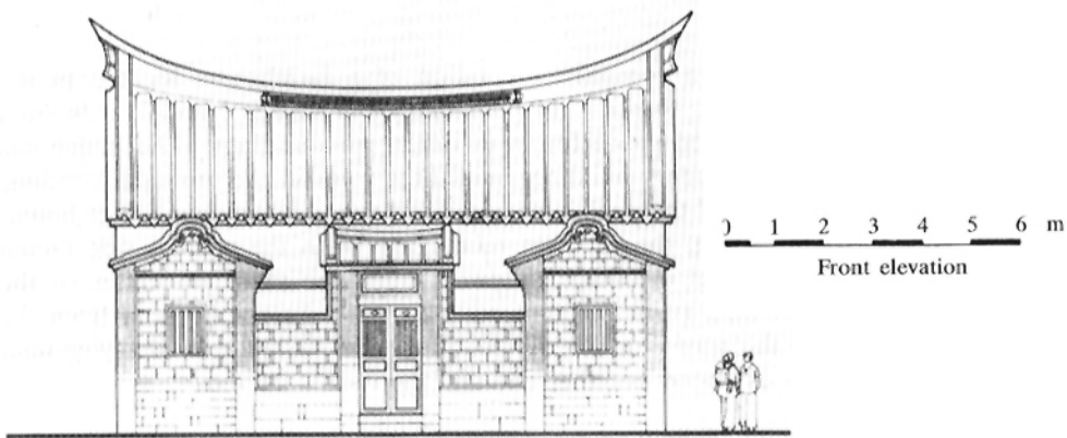
Figure 2. Front elevation of the Zhōu family house (after Dillingham and Dillingham, 1985, page 12).
