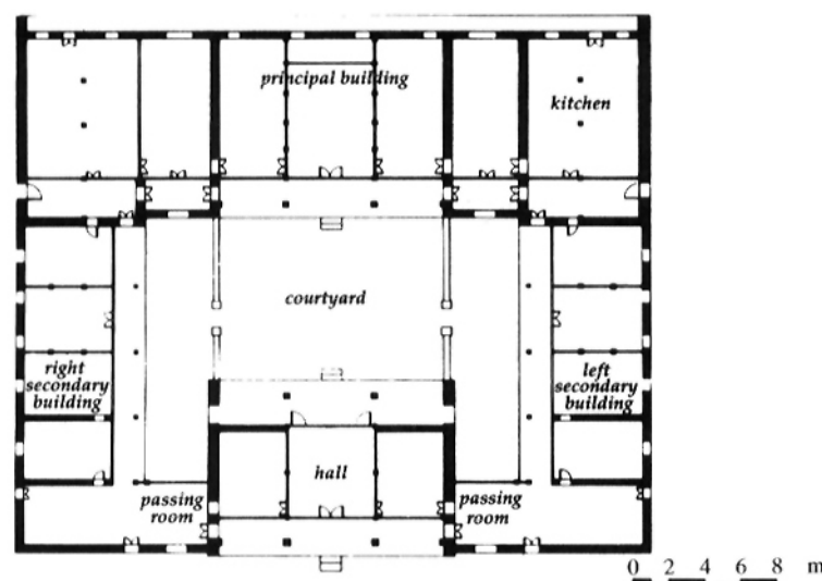
Figure 4. Plan of Dūn-běn Táng (after Lin, 1990, page 22).
