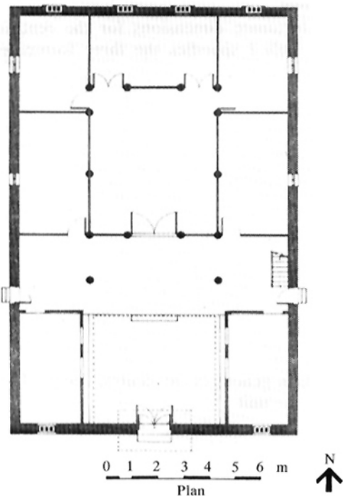
Figure 3. Plan of the Zhōu family house (after Dillingham and Dillingham, 1985, page 15).
