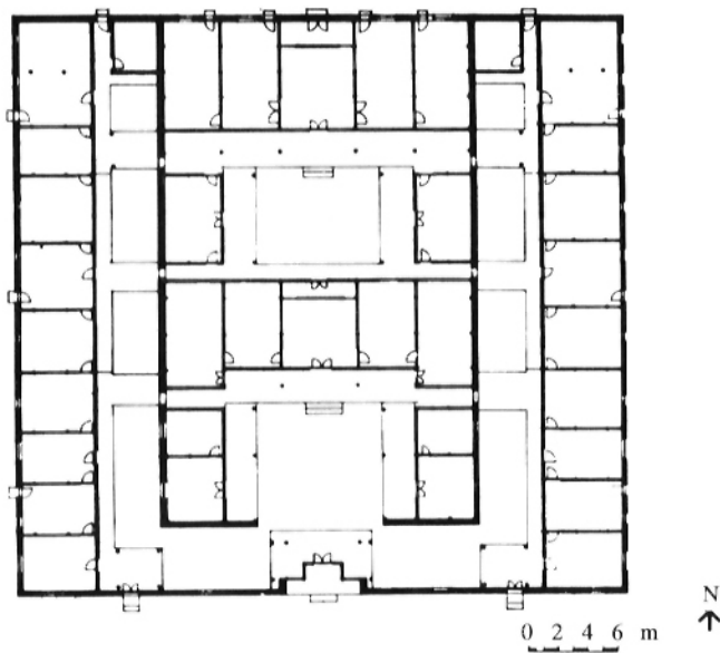
Figure 10. Plan of the Lín family great house (after Li, 1980, page 180).
