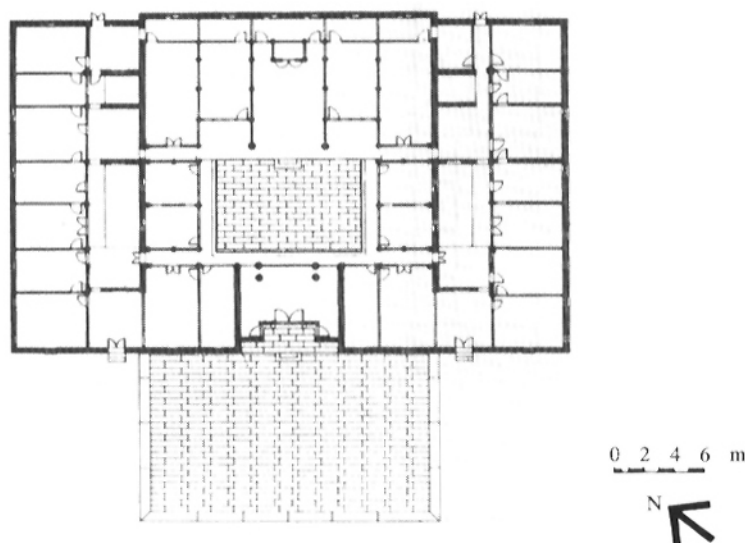
Figure 8. Plan of the Lín Ān-tài residence (after Dillingham and Dillingham, 1985, page 52).
