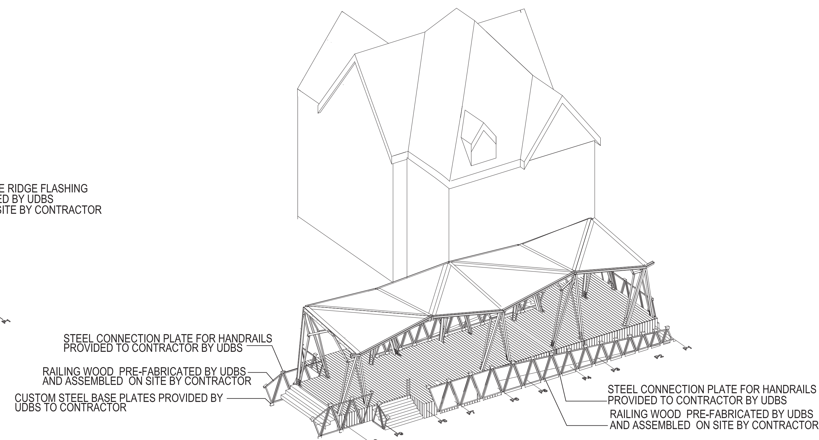
17 RAILING INSTALLATION N.T.S.
