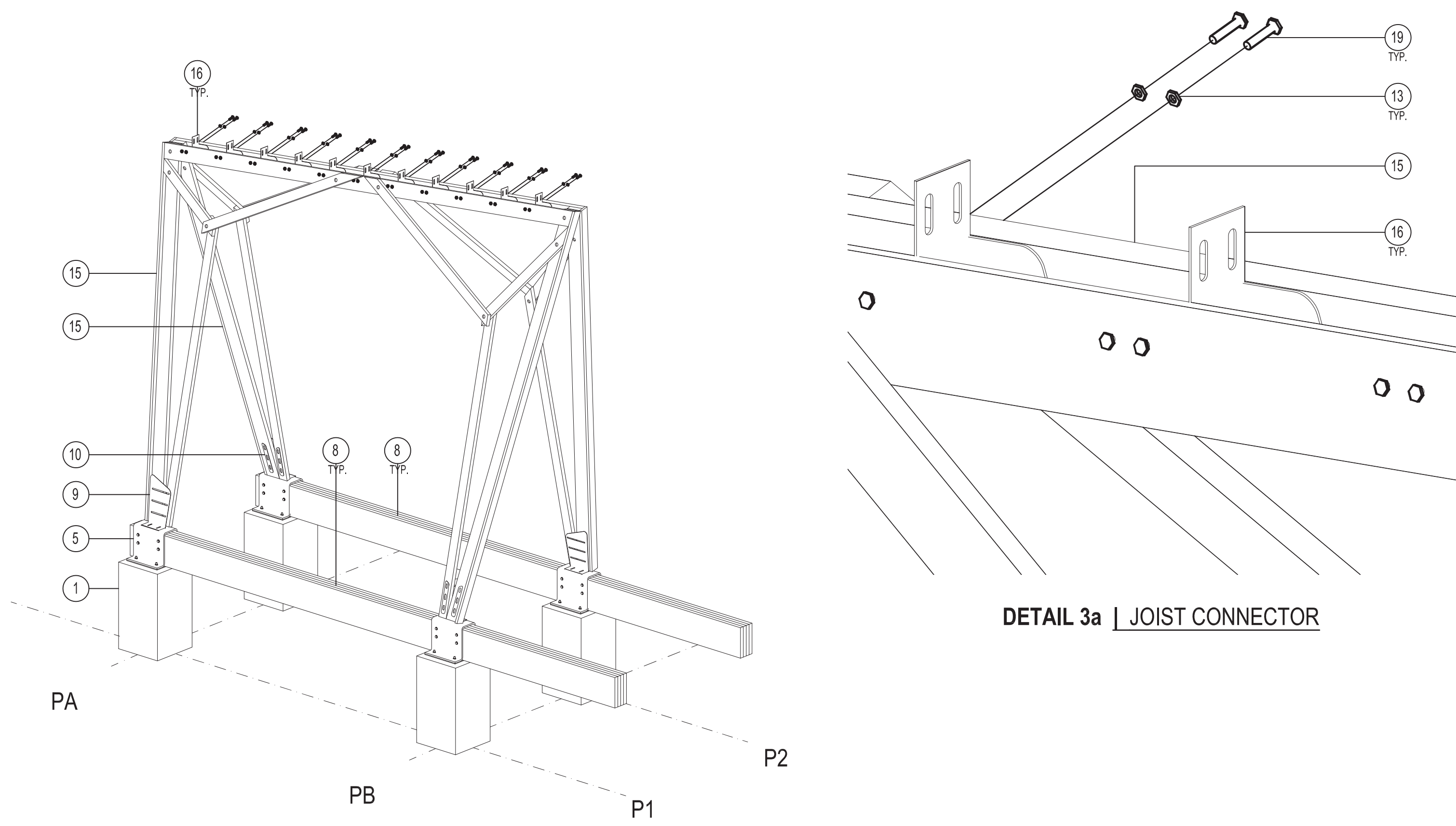
STEP 3 | FASTEN TWO FRAMES WITH ROOF JOIST CONNECTOR
