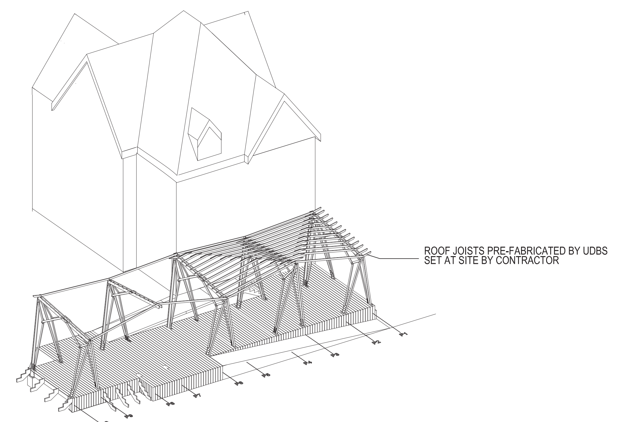
12 ROOF JOISTS BAY 01-02 N.T.S.
