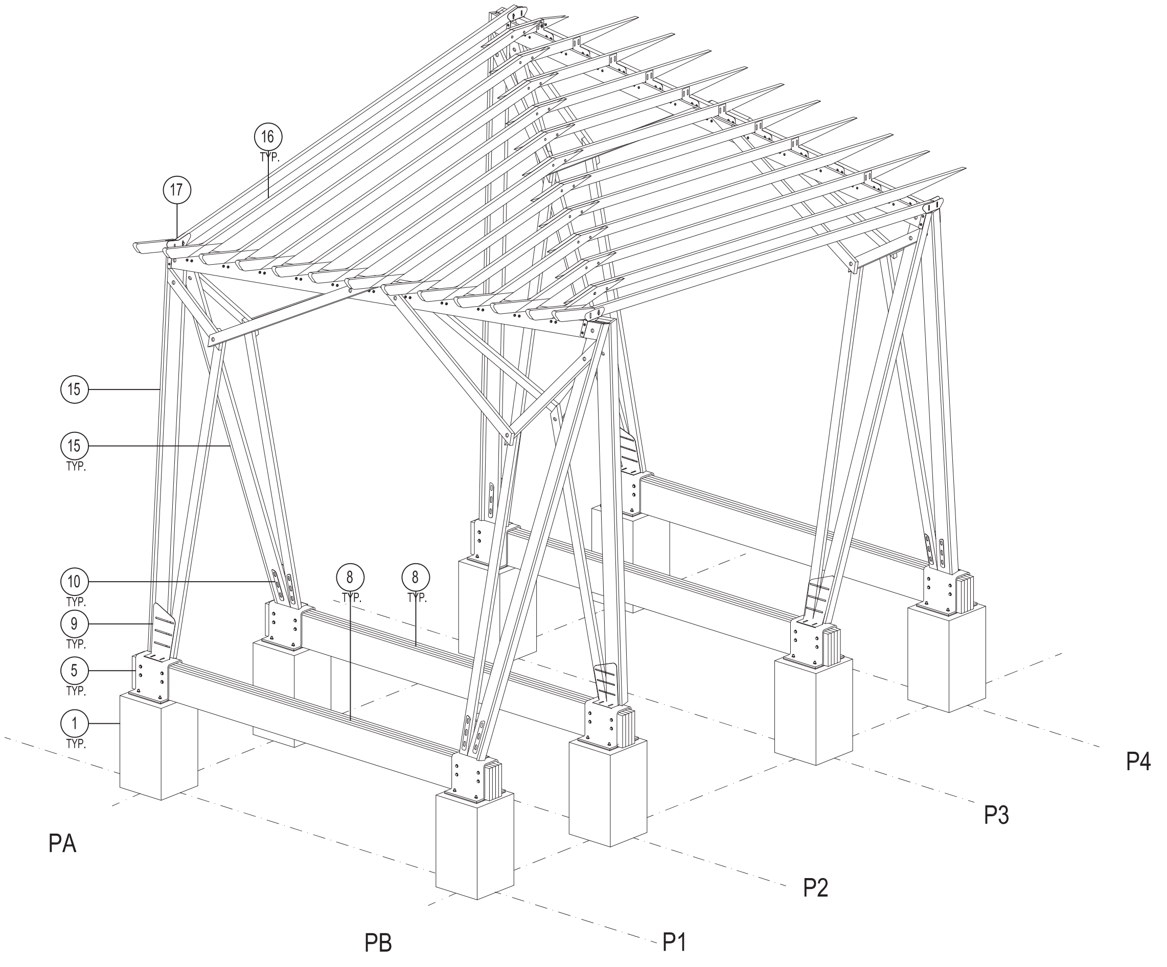
DETAIL 11 |REPEAT STEPS 8 AND 9 FOR NEXT BAY
