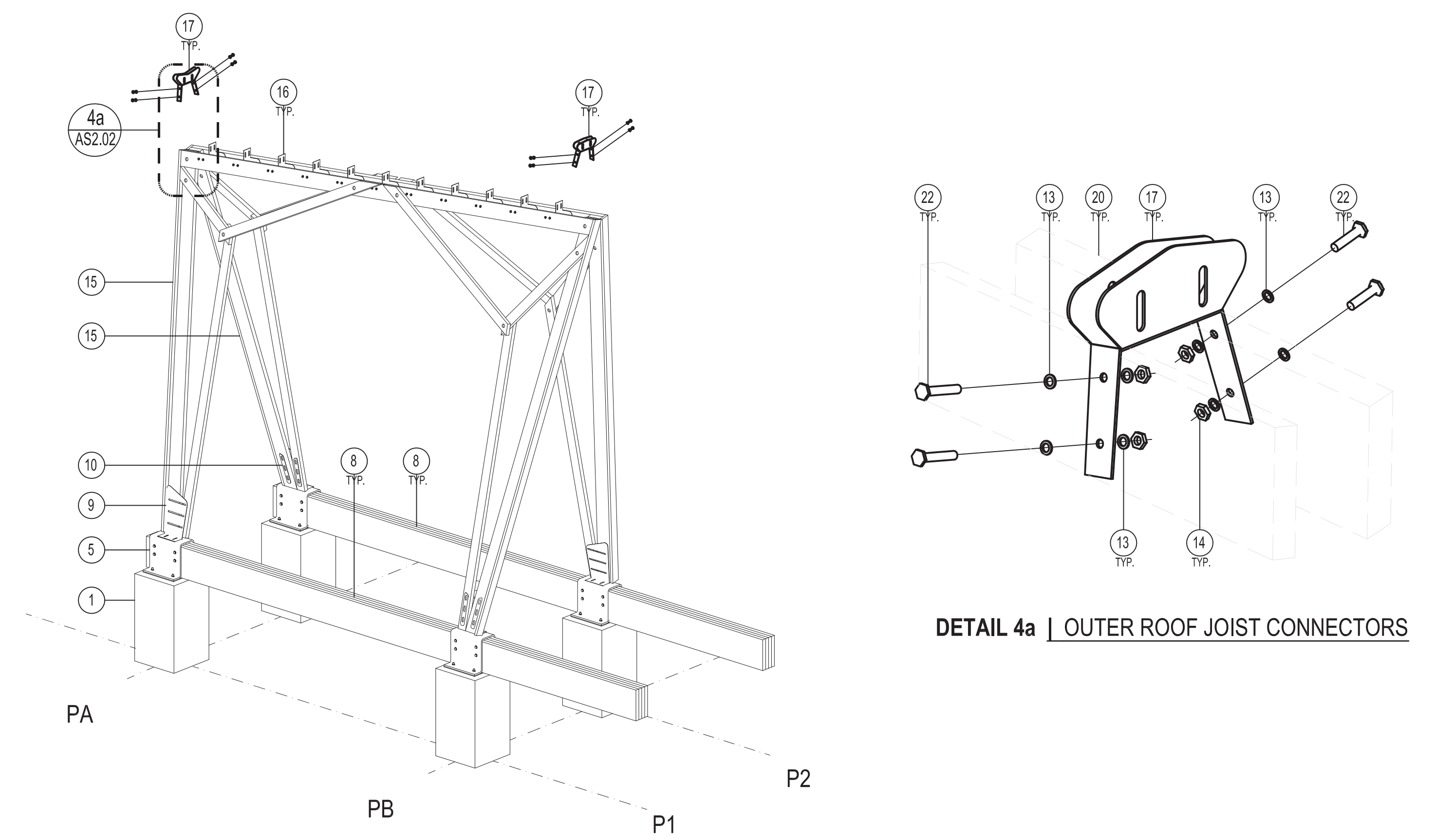
STEP 4 | FASTEN OUTER ROOF JOIST CONNECTORS
