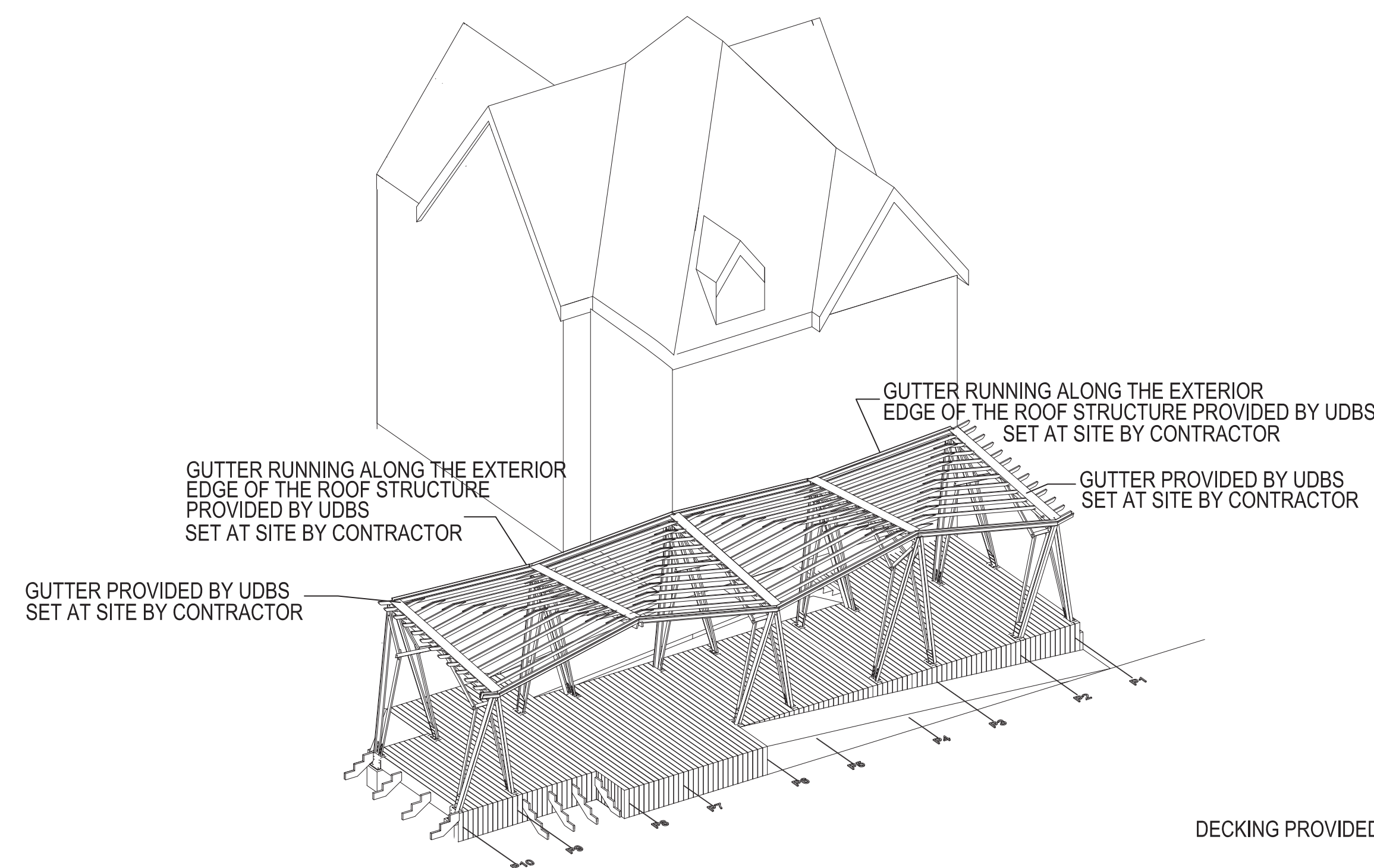
14 GUTTER AND DOWNSPOUT INSTALLATION N.T.S.
