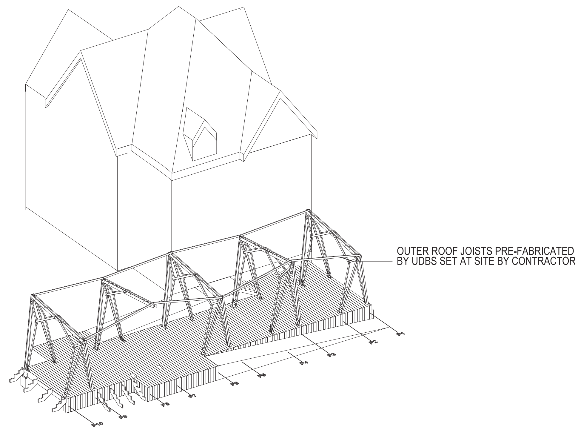
11 FRAME TO FRAME ROOF JOIST INSTALLATION N.T.S.
