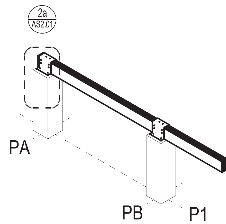
STEP 2 | DECK BEAMS AND STEEL SADDLES
