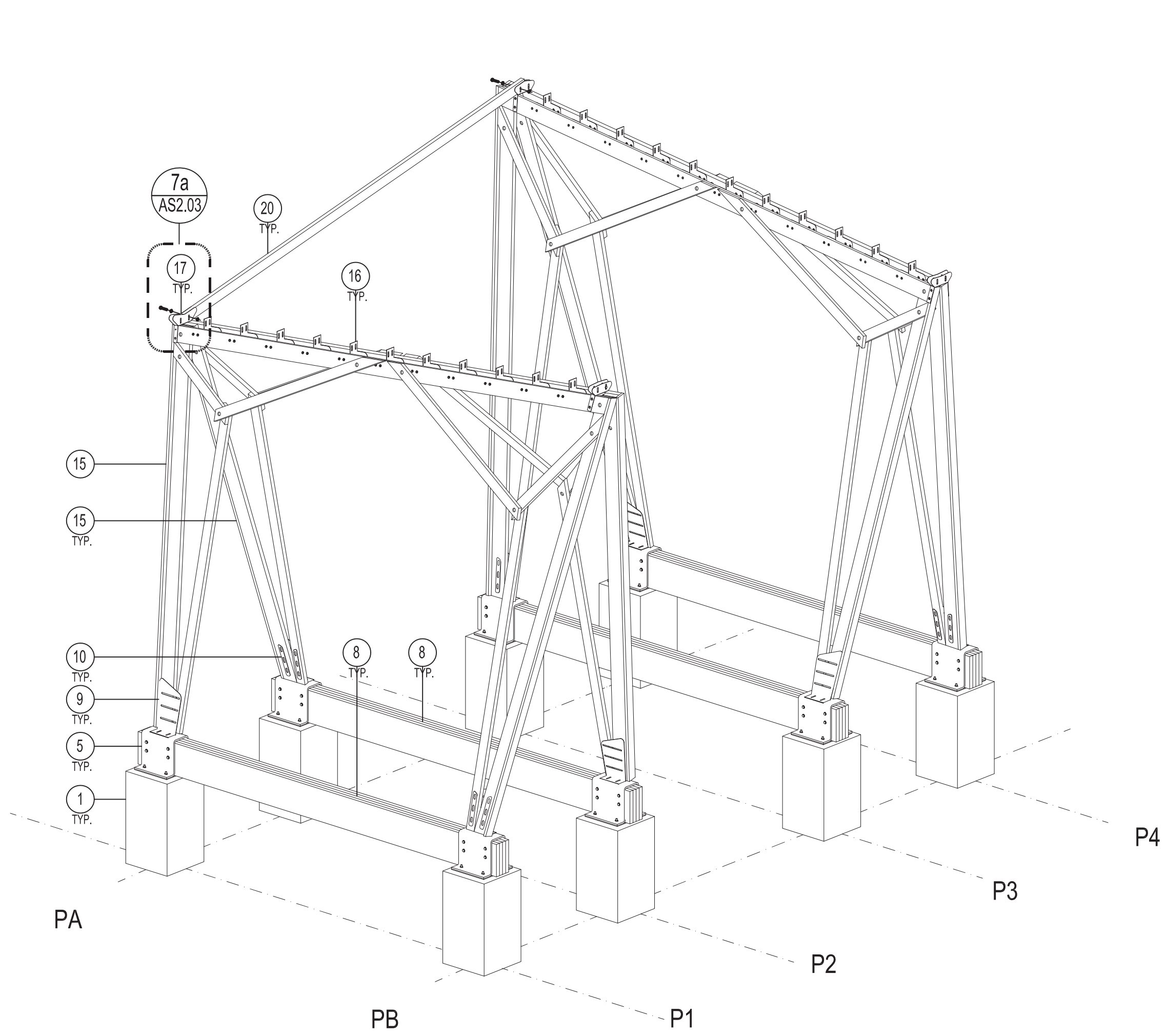
STEP 7 |FASTEN OUTER ROOF JOISTS
