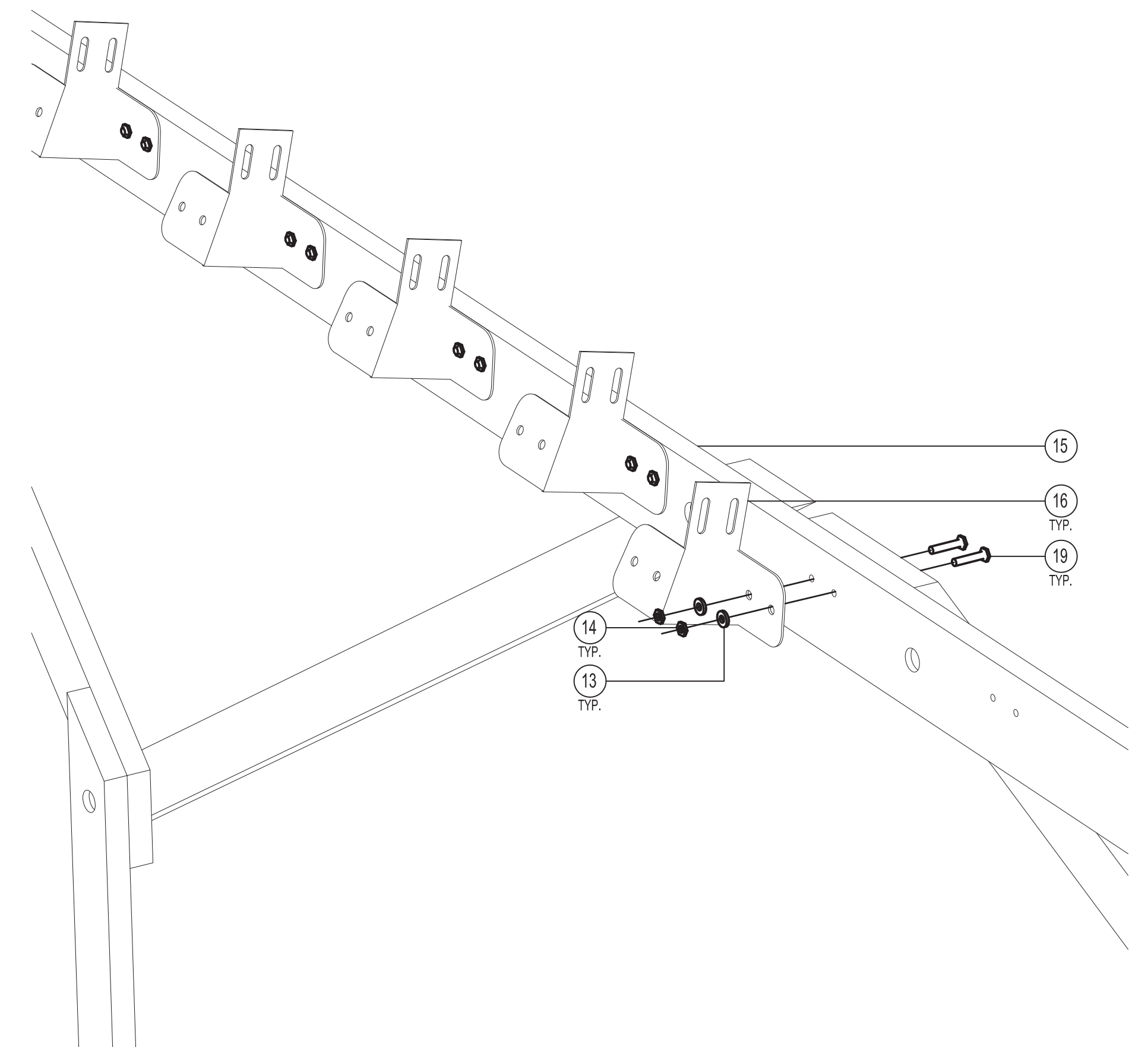
DETAIL 2a | ROOF JOIST CONNECTORS SPACED 16" O.C. (ACCORDING TO PREDRILLED HOLES)
