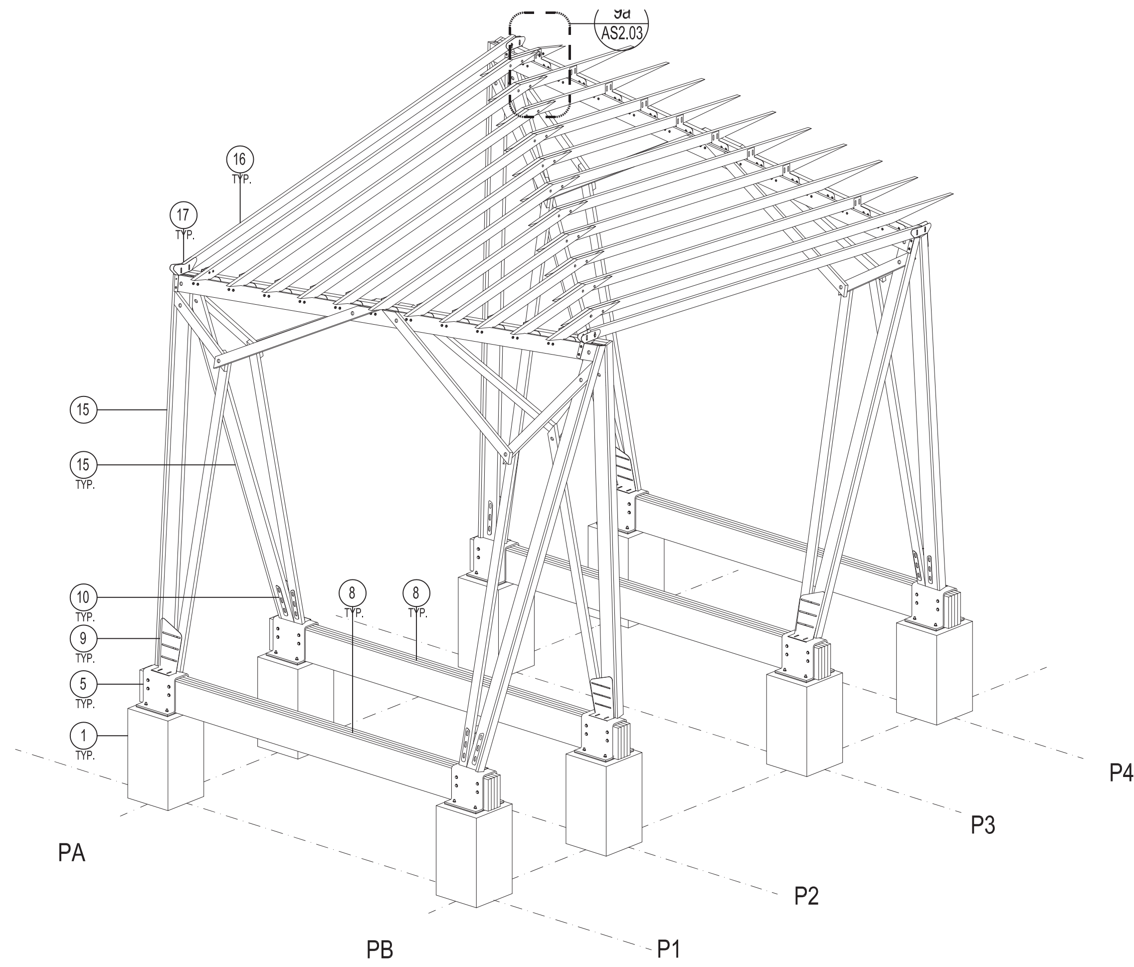
STEP 9 |FASTEN ALL ROOF JOISTS FOR ONE BAY
