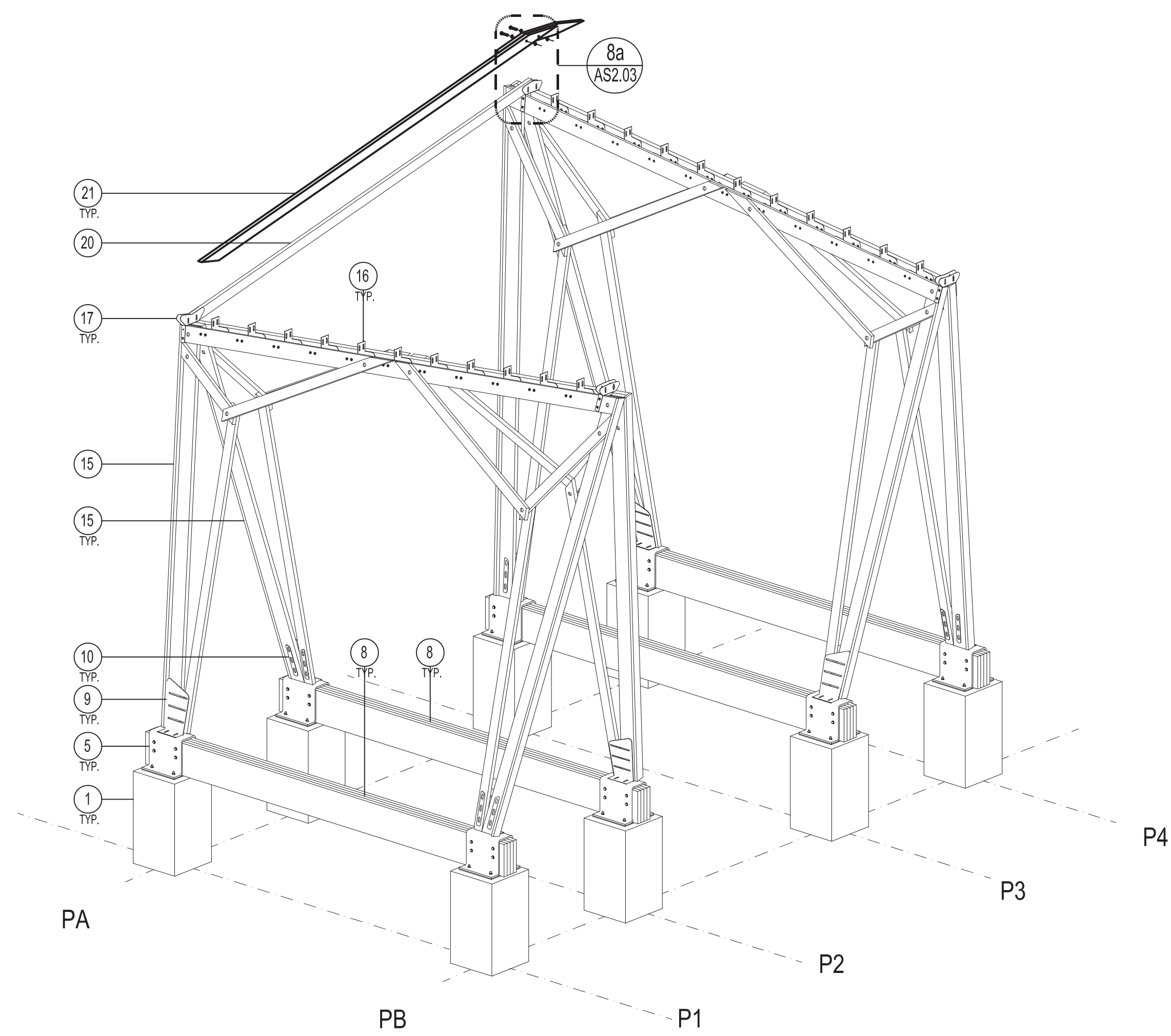
STEP 8 |UNFOLD AND FASTEN PRE-FABRICATED ROOF JOIST
