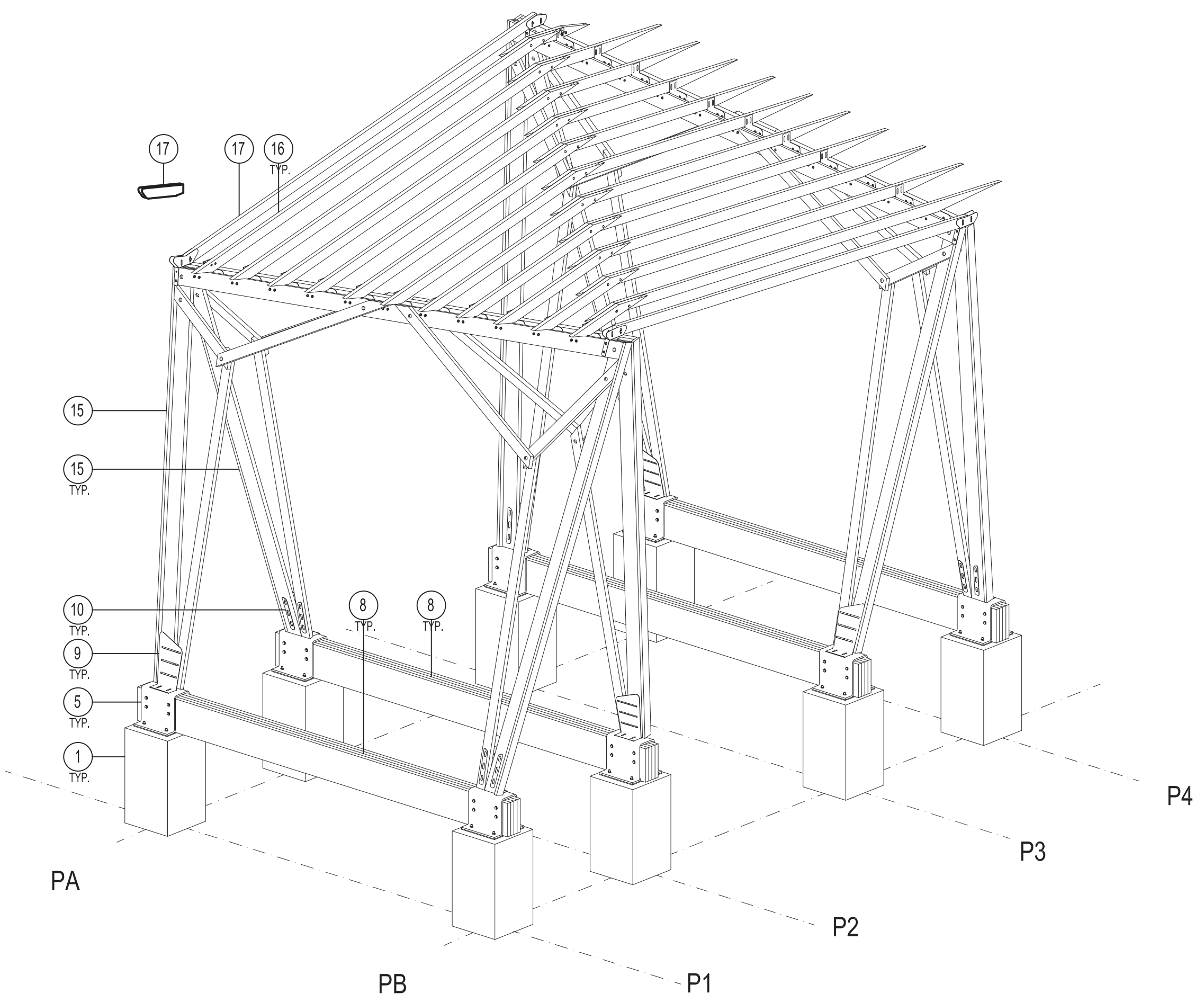
DETAIL 10 |REPEAT STEP 7 FOR NEXT BAY
