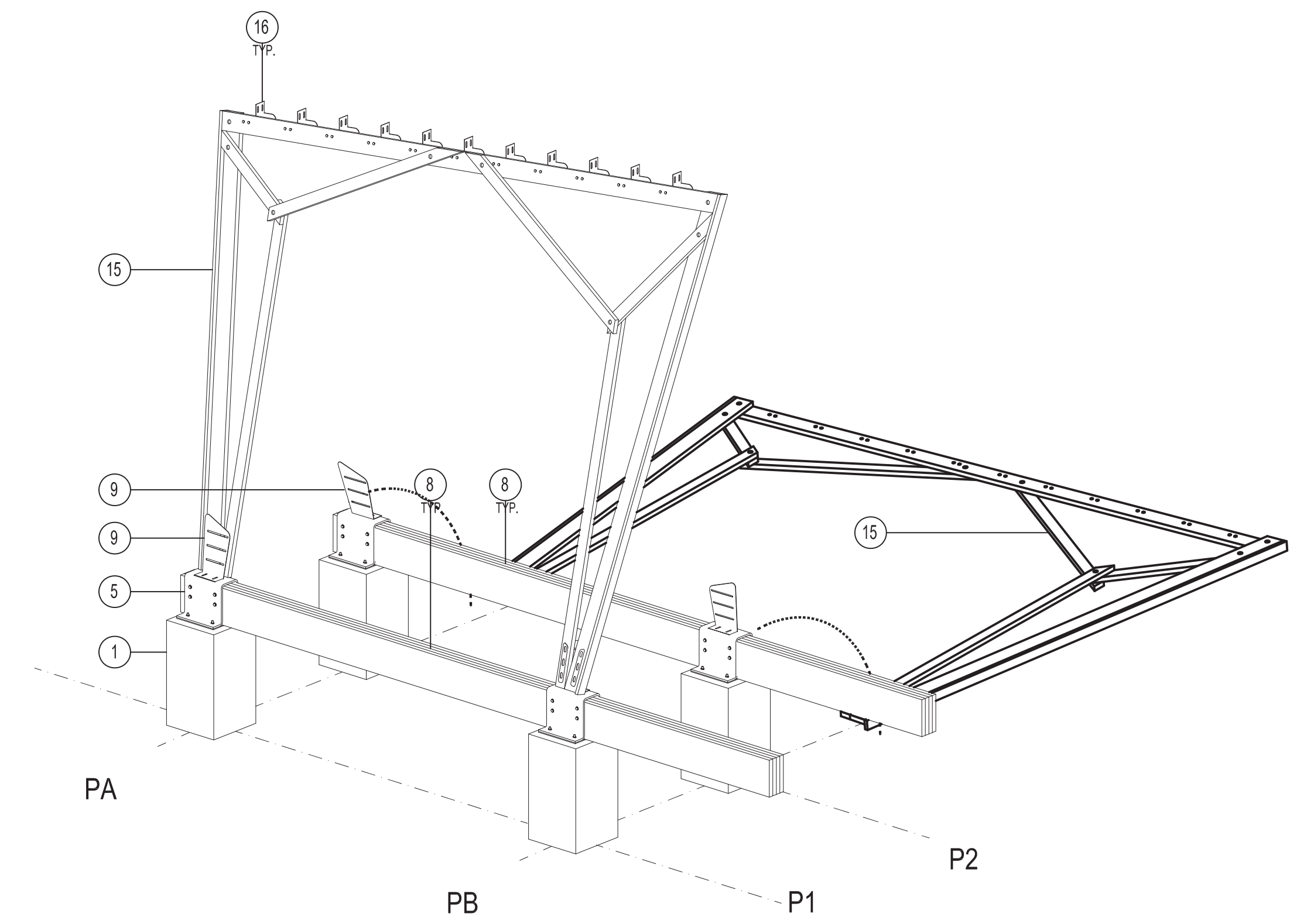
STEP 2 | ROTATE AND FASTEN FRAME "A MIRRORED" ONTO STEEL SHOES
