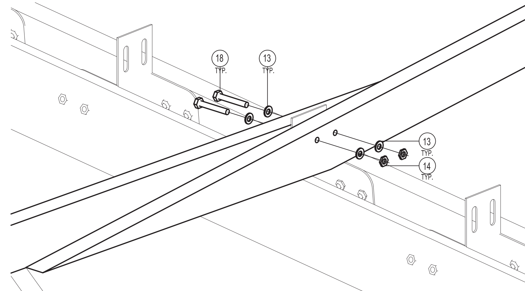
DETAIL 9a |PRE-FABRICATED ROOF JOIST TO FRAME
