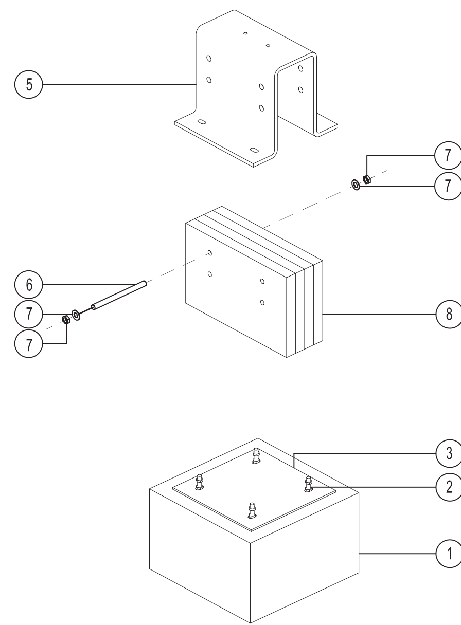
DETAIL 2a | PLACE (4) 2" X 12" BEAM AND STEEL SADDLE ON BASE PLATE
