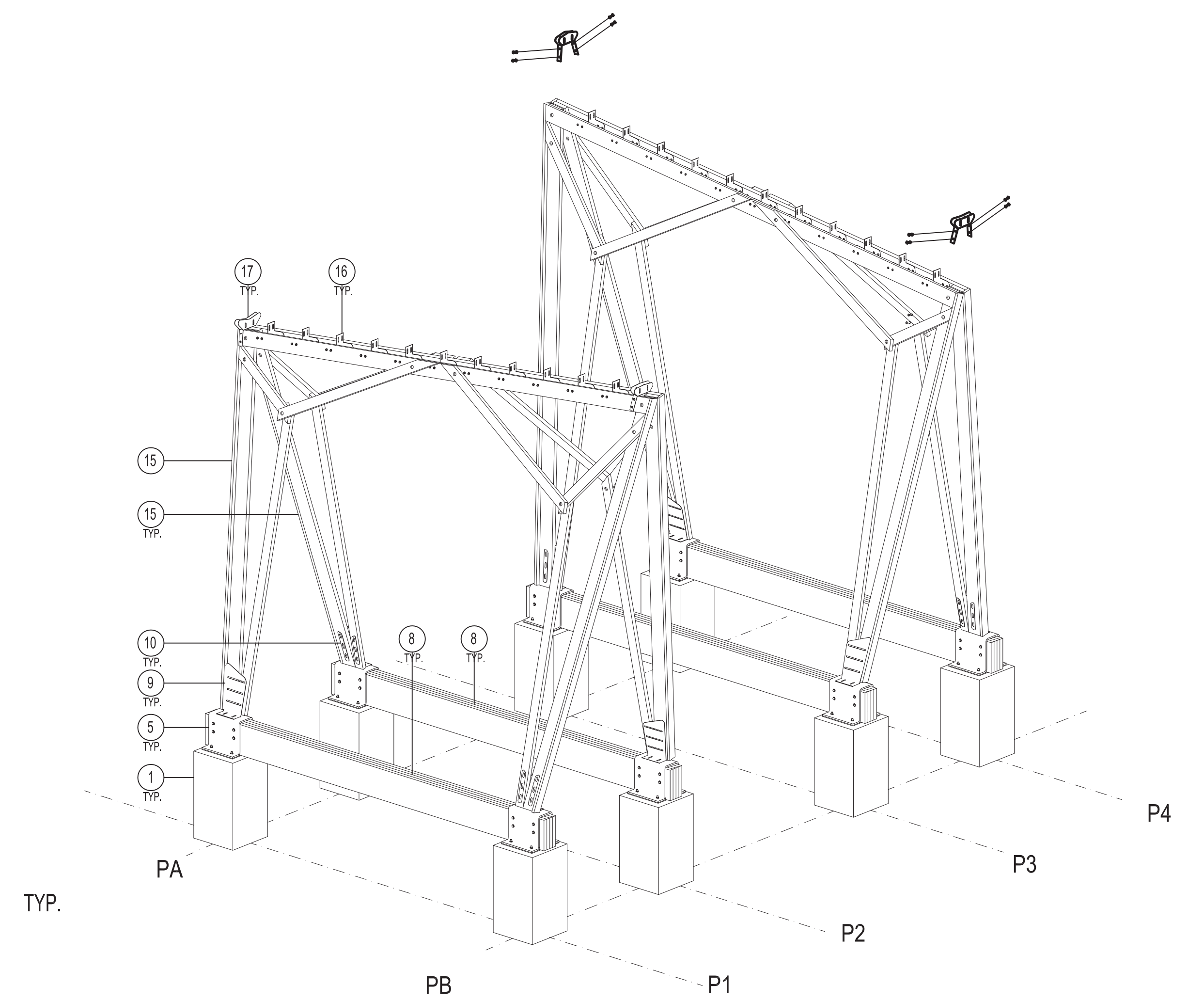
STEP 6 | FASTEN TWO FRAMES WITH ROOF JOIST CONNECTORS AND OUTER ROOF JOIST CONNECTORS
