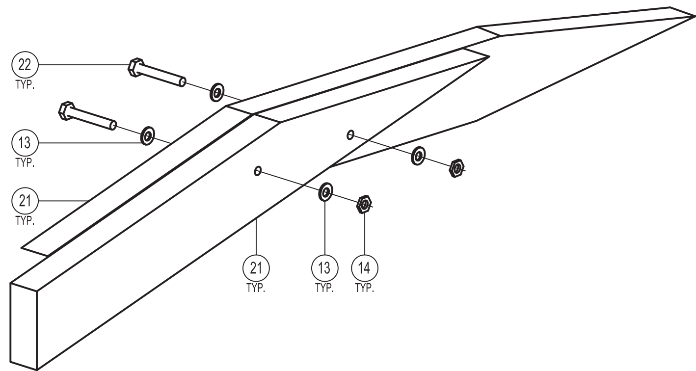
DETAIL 8a |PRE-FABRICATED ROOF JOIST
