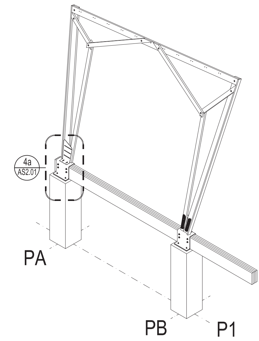
STEP 4 | FRAME
