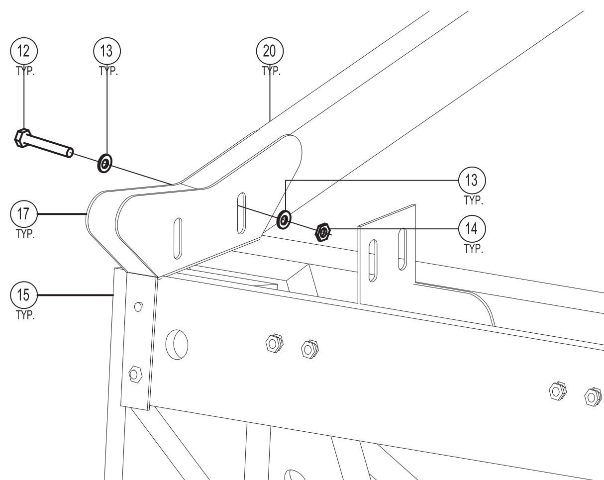
DETAIL 7a |PRE-FABRICATED OUTER ROOF JOIST
