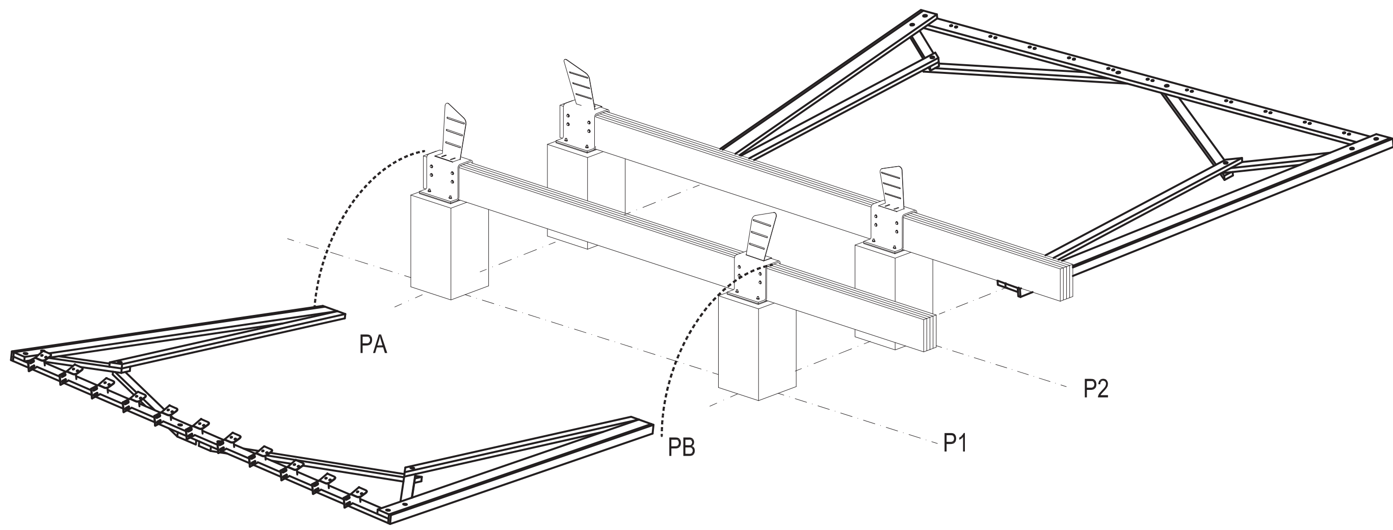
STEP 1 | ROTATE AND FASTEN FRAME "A" ONTO STEEL SHOES
