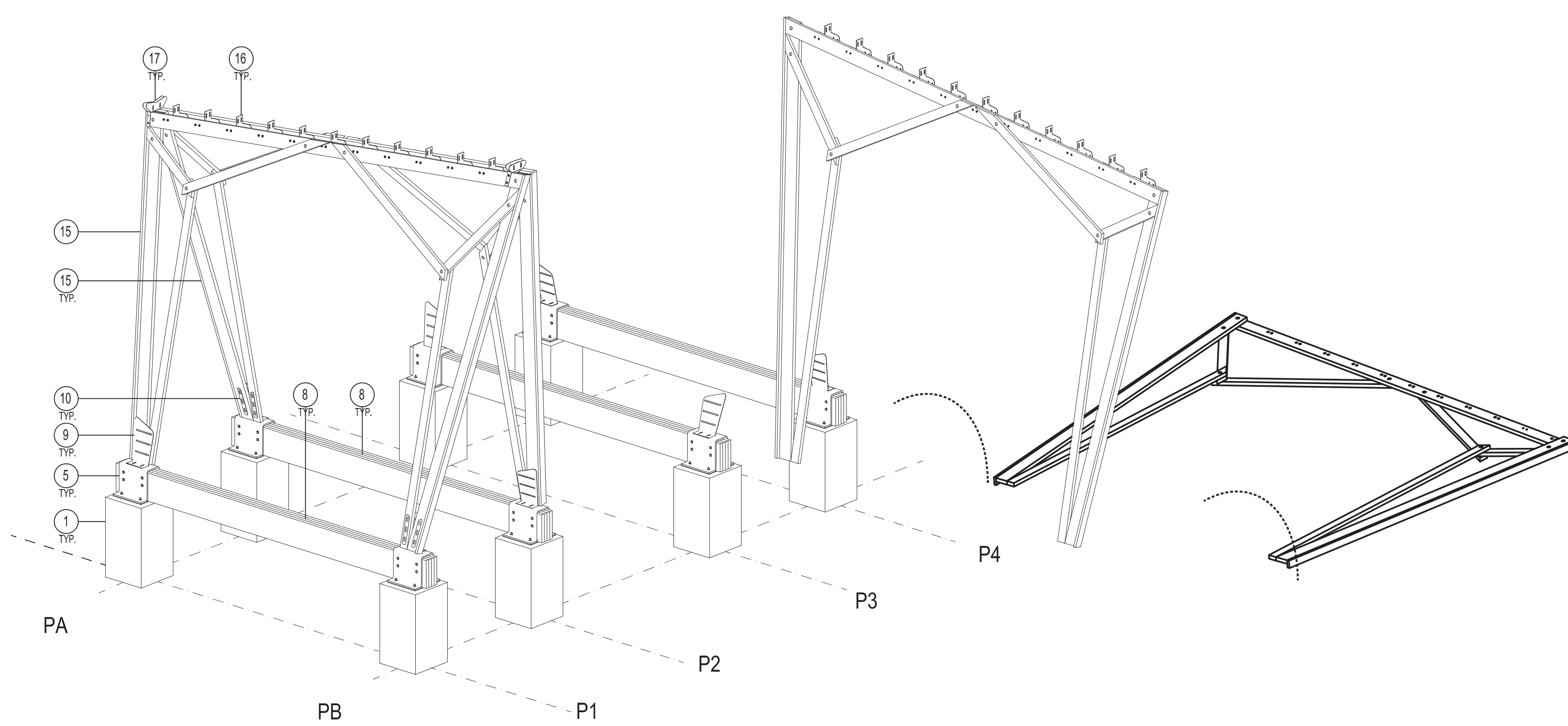
STEP 5 | ROTATE AND FASTEN FRAME "B" AND FRAME "B MIRRORED" TO STEEL SHOE
