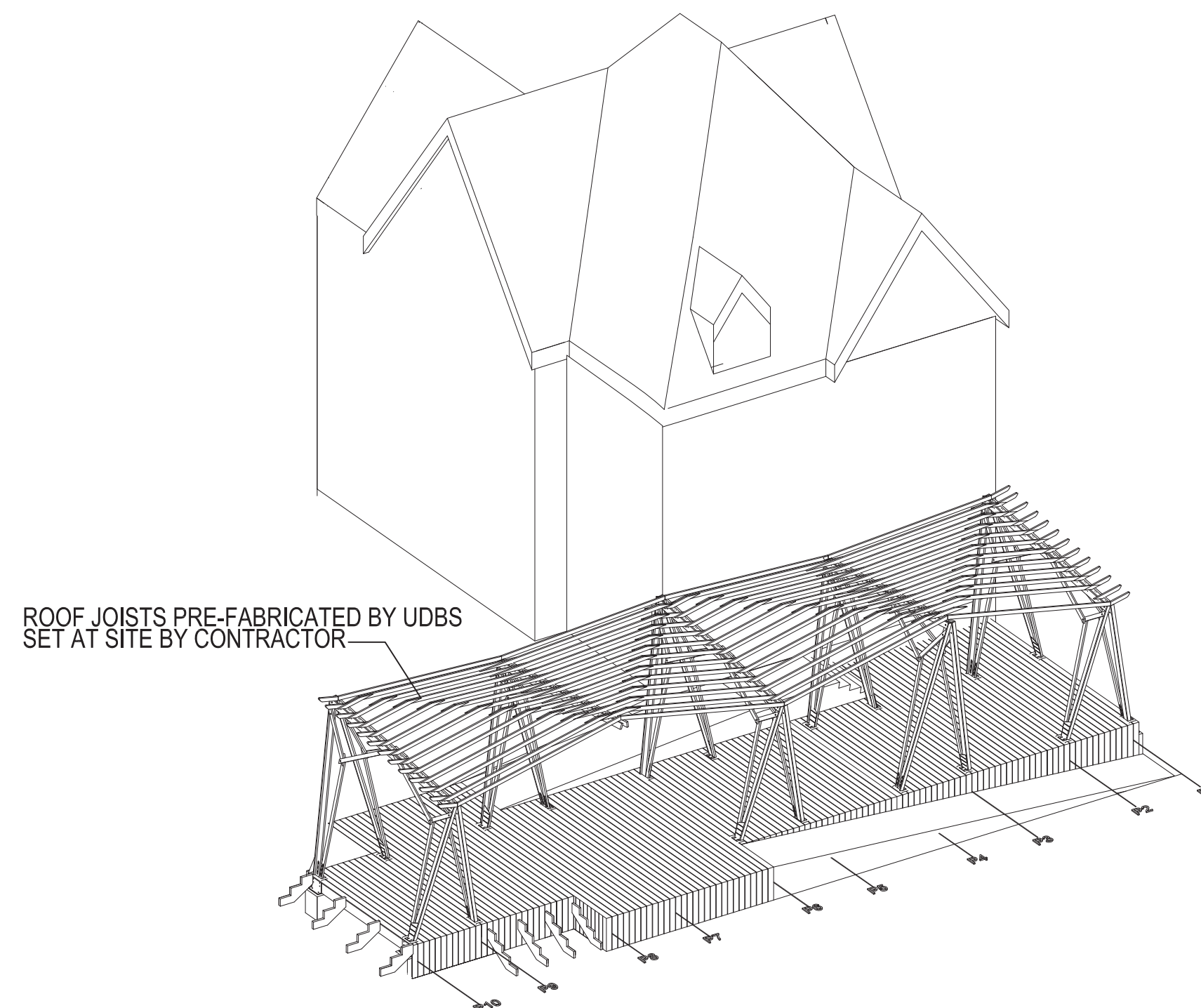
13 ROOF JOISTS BAY 03-04 N.T.S.
