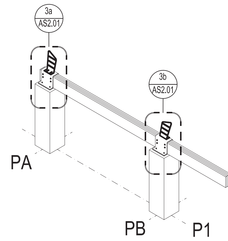
STEP 3 | STEEL SHOES
