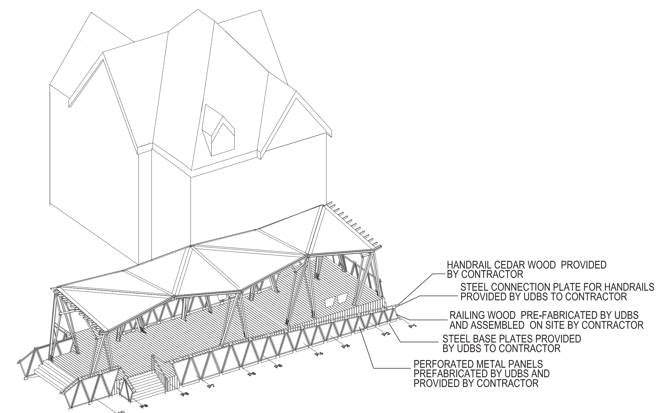
18 HANDRAIL INSTALLATION N.T.S.
