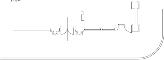
FIRST FLOOR PLAN FIRST FLOOR FACING WESTERN AVENUE
