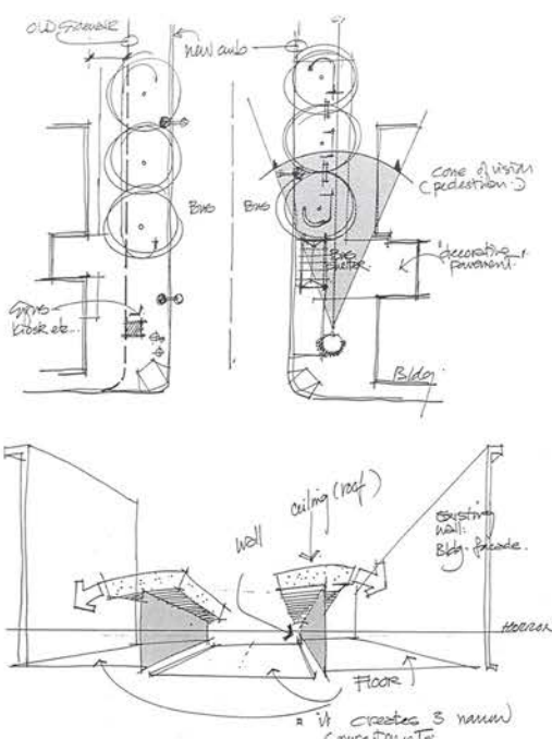
Drawing type: Sections Subject: Streetscape analysis Medium/techniques: Berol boldliners on white paper Original size: 8 1/2" x 11" Source: Wang Associates International
