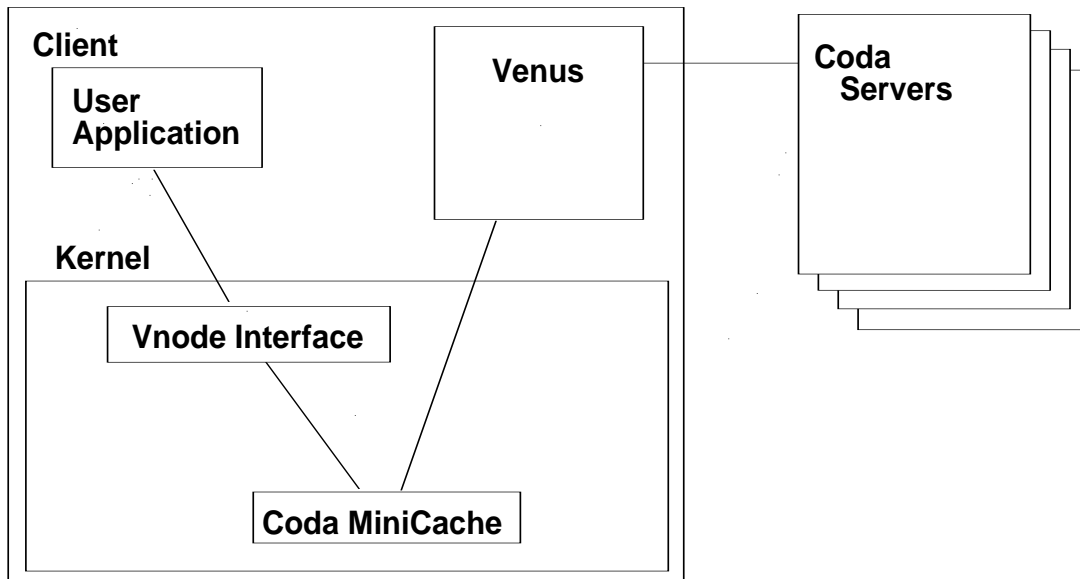
Figure 1: Coda Structure
