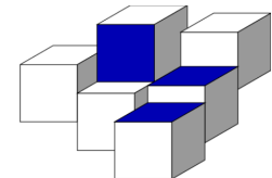
Figure 2: Three-dimensional tiling
