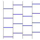
Figure 1: Two-dimensional tiling
