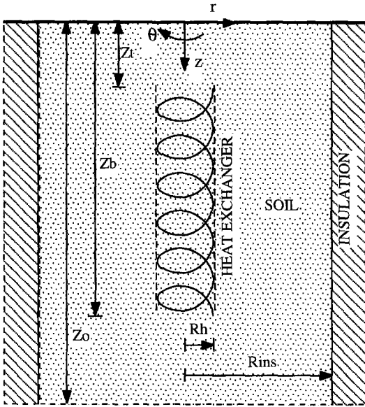
Fig. 1. Schematic description of the energy storage system.
