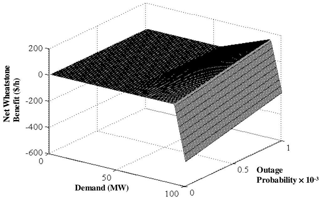
Figure 3: Expected net benefit of the Wheatstone bridge in the four-bus test network.
