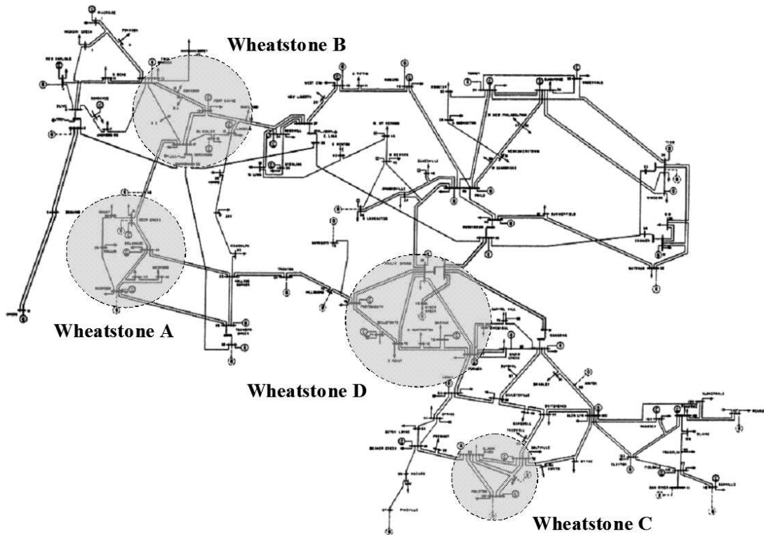
Figure 4: Four Wheatstone sub-networks of the IEEE 118-bus test network.
