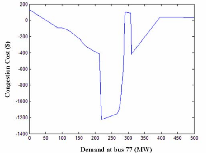
Figure 7: Congestion cost associated with Wheatstone sub-network D.
