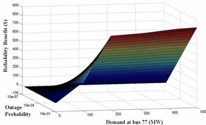
Figure 8: Monetized reliability benefit associated with Wheatstone sub-network D.
