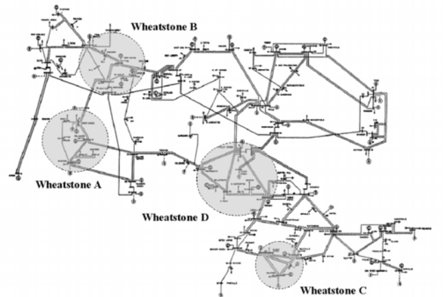
Figure 4: Four embedded Wheatstone networks in the IEEE 118-bus network.
