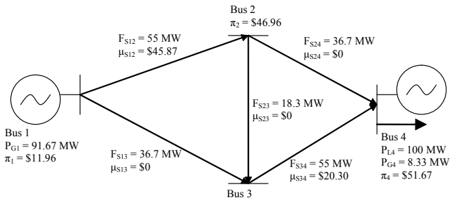
Figure 3: The four-bus Wheatstone test network.
