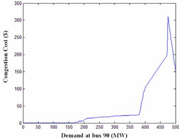
Figure 5: Congestion cost associated with Wheatstone sub-network C.
