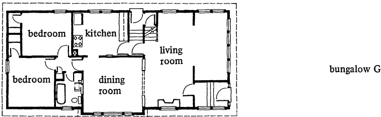
plan of first floor
