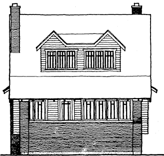
east elevation
