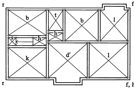
Figure 11. Shape C_4 generated from shape C_3 by two applications of schema 11.
