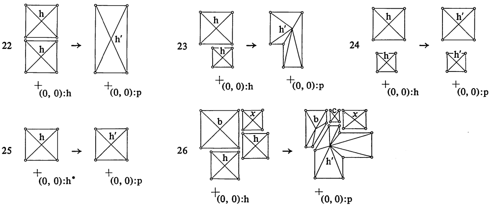
Figure 15. Schemata to merge two halls or to confirm the existence of halls which cannot be merged.
