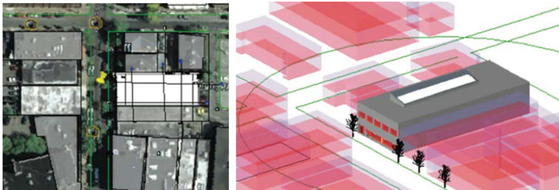
FIGURE 15. Test Case, Site plan and massing (left), 3D view (right).
