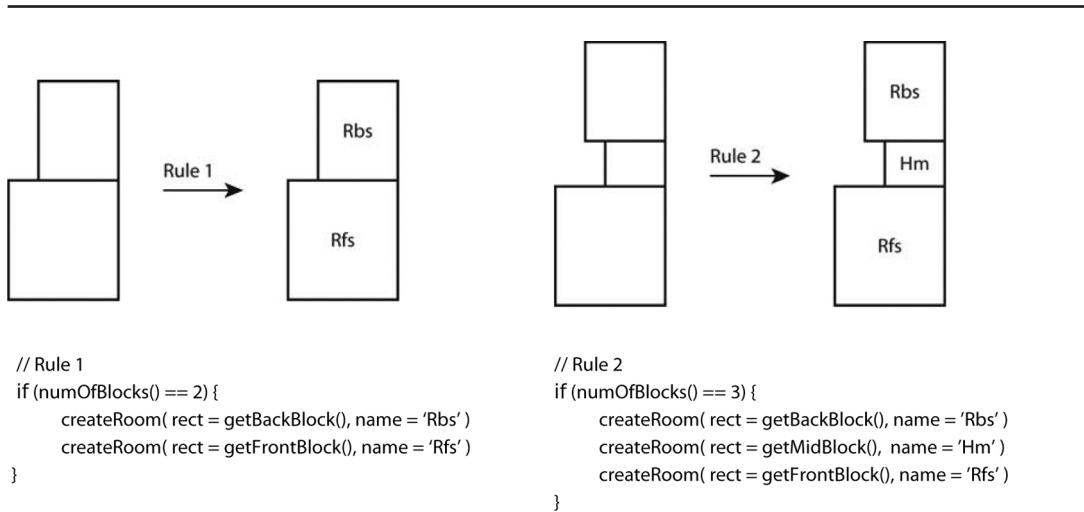
Figure 9. Naming the blocks: rules 1 and 2.
