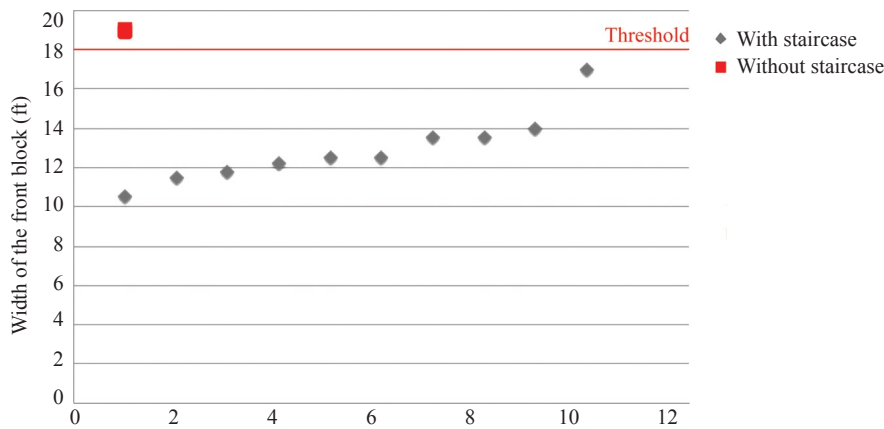
Figure 15. [In colour online.] Distribution of widths used in quantifying the shape rules generating staircases.
