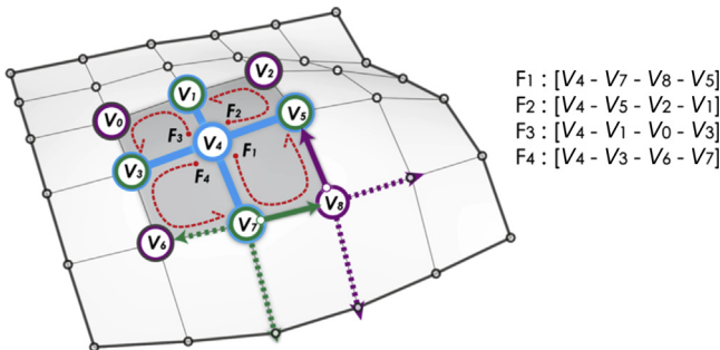
Figure 8 Fitting mesh faces by shortest path search.
