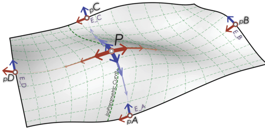
Figure 5 Conjugate curves derived from boundary-driven computation and underlying isoparametric grid.
