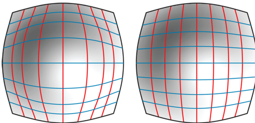
Figure 3 Two types of surface subdivision (left) uniform iso-parametric intervals (right) optimizing face sizes via equidimensional intervals.
