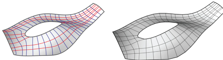
Figure 14 (Left) conjugate curve network (right) preliminary BDMesh .
