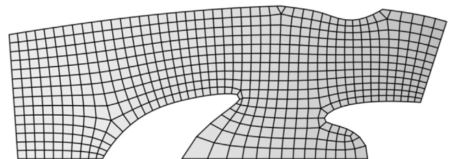
Figure 18 Optimized BDMesh for the western façade of the Next-Gen Museum (Hadid, 2008).
