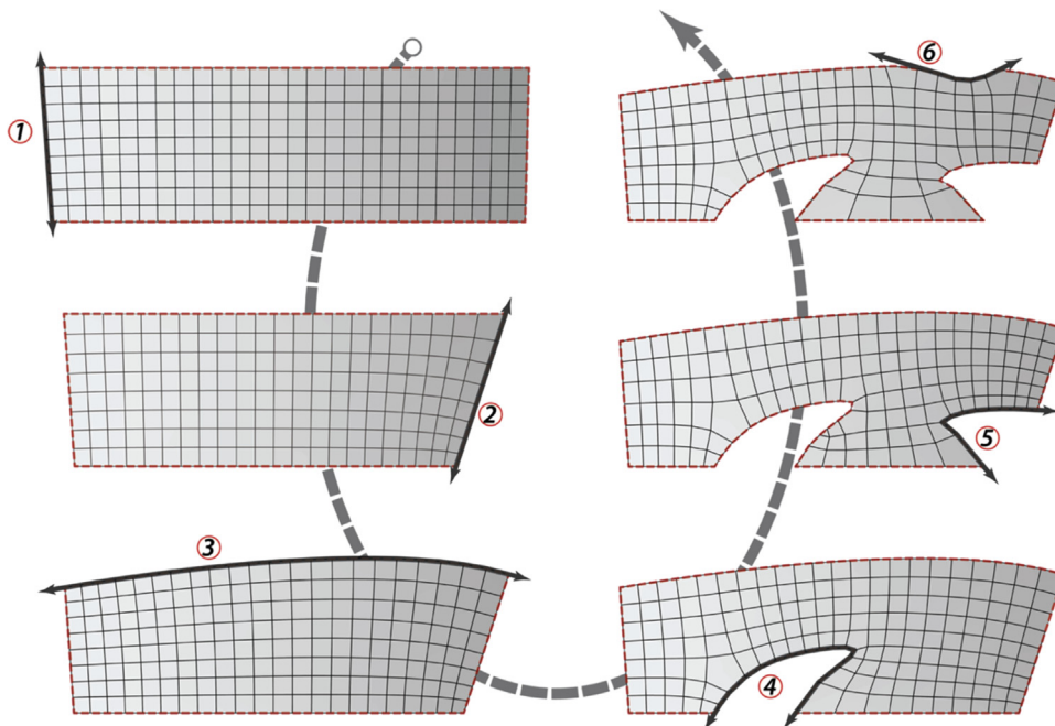
Figure 17 Variations of BDMesh results ranging from single to multiple boundary conditions.
