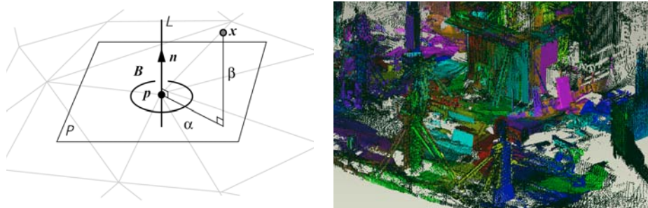
Figure 2. Left: An oriented point basis created at a vertex in a surface mesh, reproduced from (Johnson, 1997). Right: A registered as-built model overlaid with an as-design model.
