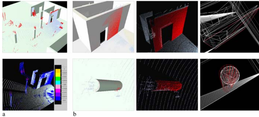
Figure 4. (a) Top : Clutter identified, shown in red. Bottom : Deviation color analysis of a scan. (b) Top : Fitting an infinite plane (Results: angles with X-Y- and Z-axes = 89.4438^\circ , 0.5443^\circ , 0.1146^\circ respectively. Ground truth: is in Y-Z plane). Bottom : Fitting an infinite cylinder (Results: radius = 28.21cm. Ground truth: 25.53cm)
