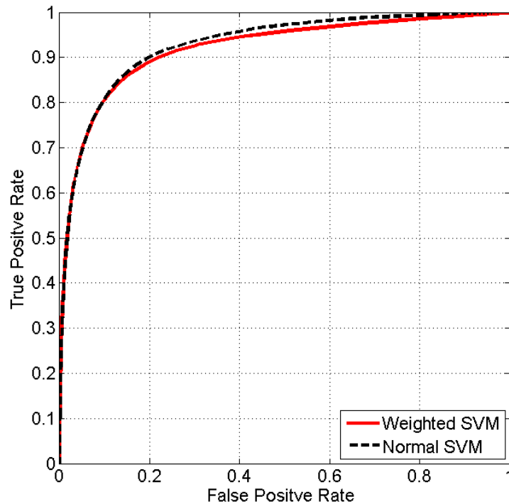
Figure 5: ROC curves of two different methods. Weighted SVM performs as well as normal SVM while using a much smaller number of pixels.
