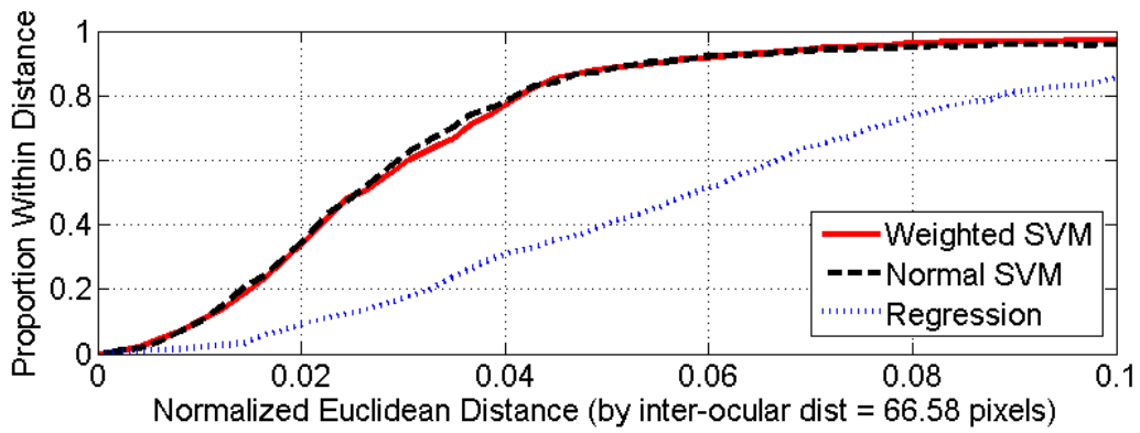
Figure 4: Distance threshold versus the proportion of iris localization within the threshold. The distance is taken as the Euclidean distance from the ground truth landmark to the predicted iris location normalized by the inter-ocular distance. Weighted SVM performs as well as the other method while using a much smaller number of pixels. The Regression curve is the result of using initial guess produced by the linear regression predictor.
