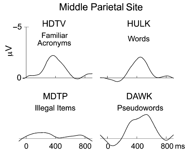
Fig. 1. Grand-average difference waves (first minus second presentation) for familiar acronyms, words, pseudowords, and illegal strings at the middle parietal channel (with an example from each stimulus category indicated above the category name).
