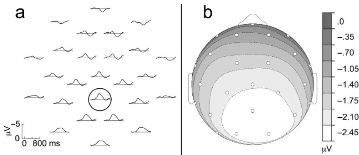
Fig. 3. Familiar-acronym repetition effect. Grand-average repetition-effect difference waves for familiar acronyms at all 26 scalp channels are displayed in (a), with the middle parietal waveform circled. The distribution of the effect (top view of the head) between 325 and 375 ms after stimulus onset is shown in (b).
