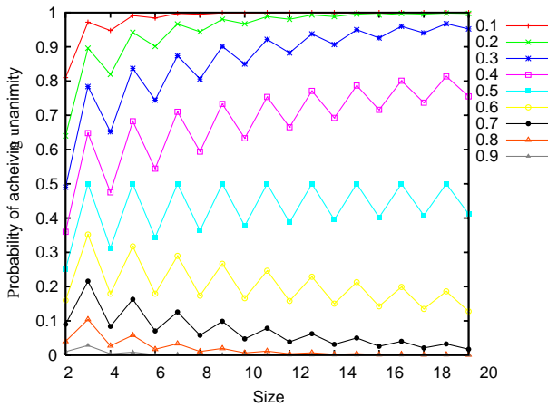
Fig. 2 Complete networks for 9 error probabilities
