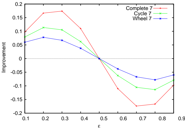
Fig. 11 Comparing the three networks and individual reliability
