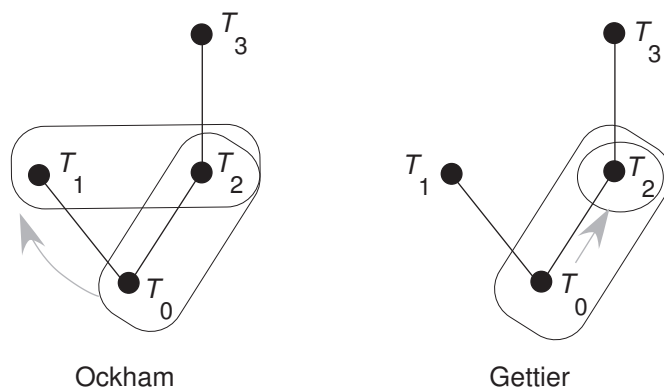
Figure 15: Gettier counterexample to Ockham efficiency
