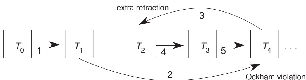
Figure 12: Ockham violator's extra retraction
