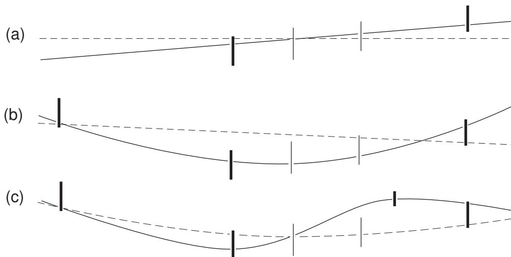
Figure 10: first, second, and third order effects
