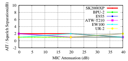
Figure 6: Audible interference threshold (AIT) remains stable when varying mic signal atten.
