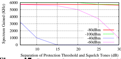
Figure 17: Impact of protection threshold.
