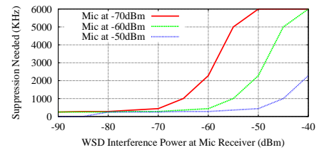
Figure 3: Suppression needed by WSD.
