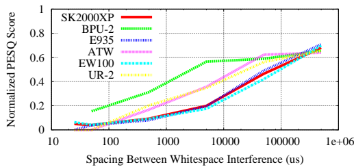
Figure 11: Resulting interference with variable spacing.
