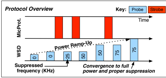
Figure 14: Overview of SEISMIC adaptation protocol.
