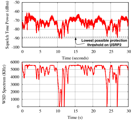
Figure 23: In the more challenging scenario, the WSD is able to avoid mic disruption, even at low mic powers, showing robustness.
