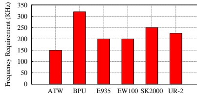
Figure 8: The frequency tolerance thresholds for all of the mics for no audible interference.
