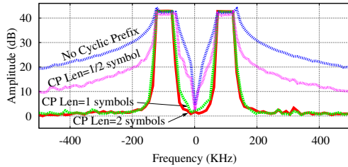
Figure 16: Strokes with varying CP in the frequency-domain.
