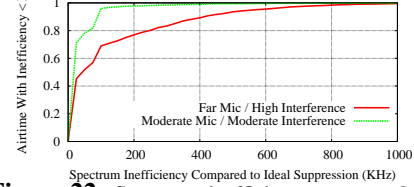
Figure 22: Spectrum inefficiency compared to ideal suppression as a fraction of airtime.
