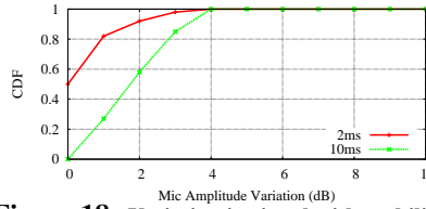
Figure 18: Variation in signal with mobility.
