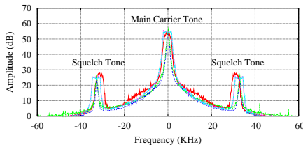
Figure 1: Spectrum signature of 6 idle mics.
