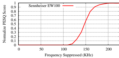
Figure 7: Senn. EW100 requires 200KHz of non-interfering noise for no audible interference.
