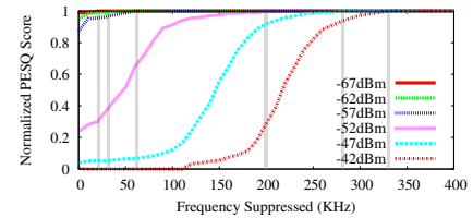
Figure 9: Varying WSD interf. power at mic receiver, suppression needed varies greatly.
