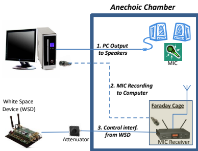
Figure 10: Anechoic chamber setup for audible interference tests.
