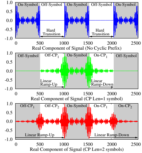
Figure 15: Strobes with varying cyclic prefixes in the time-domain.
