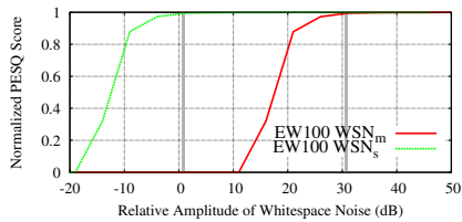
Figure 4: Audible interference, varying WSN. Areas where score reaches 1 are highlighted.
