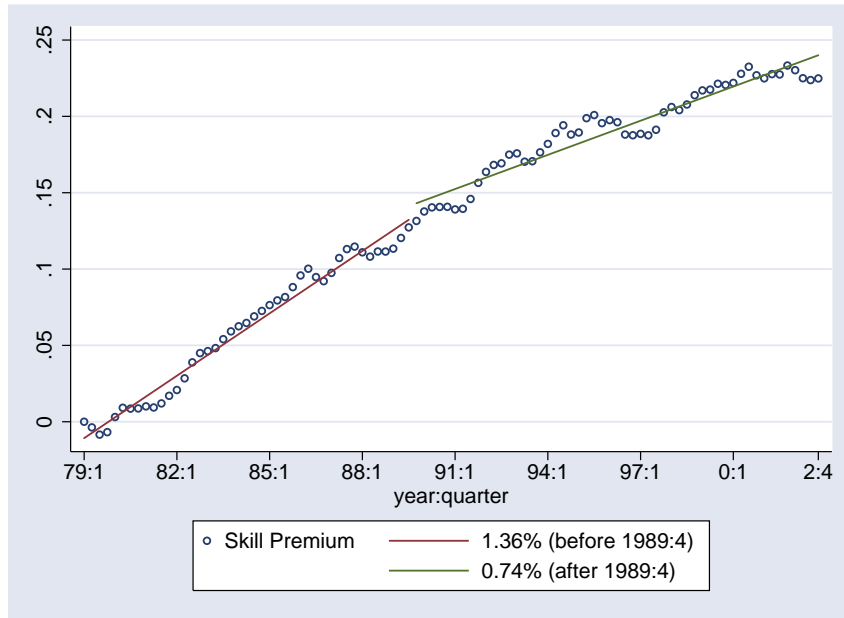
Figure 5: Skill premium
