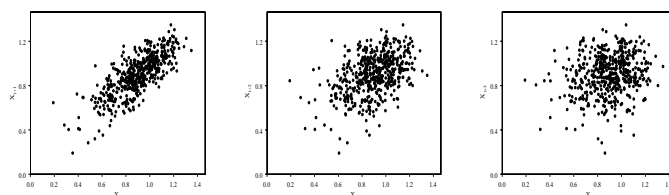
Figure 7: Scatter Plots of (x_t, x_{t+1}) , (x_t, x_{t+2}) , and (x_t, x_{t+3}) for the Artafit Data
