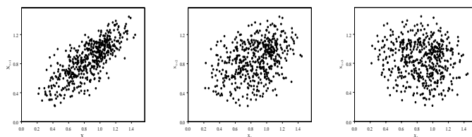
Figure 6: Scatter Plots of (x_t, x_{t+1}) , (x_t, x_{t+2}) , (x_t, x_{t+3}) for the Artifact Data
