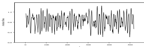
Figure 3: Time-series Plot of the Artifacts Data
