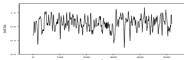
Figure 4: Time-series Plot of the Artafit Data
