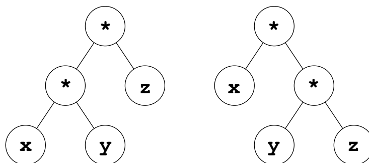
Figure B.2: Left and right associativity of x \star y \star z
