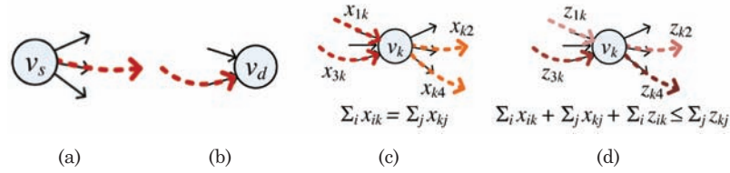
Fig. 4. (a) Flow constraints at the starting node; (b) flow constraints at the ending node; (c) conservation constraints at an intermediate node; (d) progression constraints at an intermediate node.
