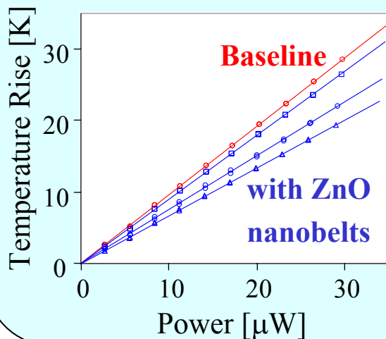
Thermal Resistance
