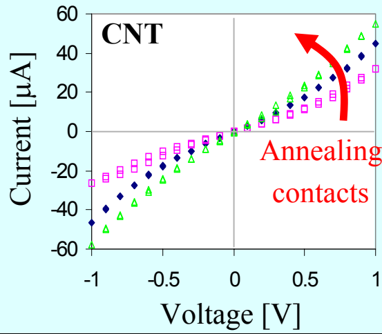
Electrical Resistance
