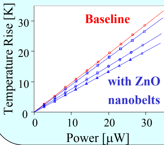
Thermal Resistance
