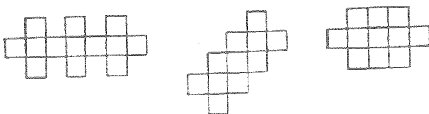
Figure 16. Three shapes in the class determined by the recursive definition of section 2.2, when used in conjunction with the spatial relation specified by the decomposition of figure 15(b).
