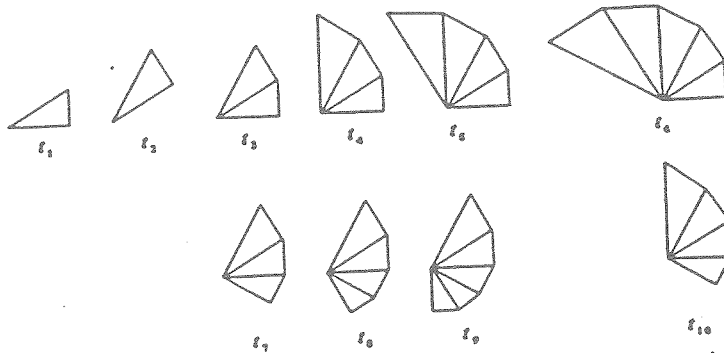
Figure 3. Some shapes in the class defined recursively using the spatial relation specified by the set of shapes \{t_1, t_2\} .
