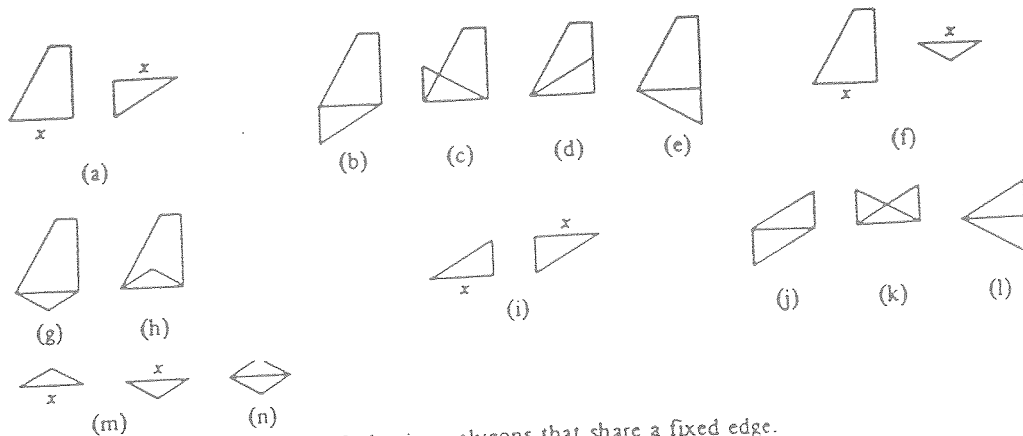
Figure 7. Spatial relations specified using polygons that share a fixed edge.
