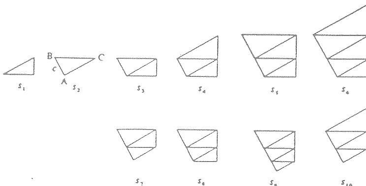
Figure 2. Some shapes in the class defined recursively using the spatial relation specified by the set of shapes \{s_1, s_2\} .
