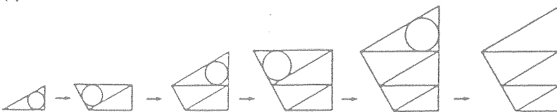
Figure 4. A shape grammar and the generation of a shape.
