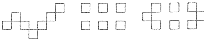
Figure 18. A shape grammar defined in terms of the spatial relations given in figures 17(a) and (b); two generations of the shape drawn in figure 13(a) using this shape grammar; and three additional shapes in the language defined by this shape grammar.
