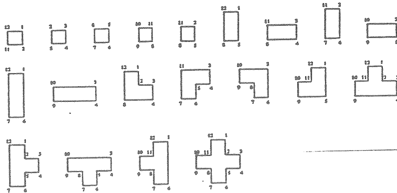
Figure 14. The twenty polygons in the shape drawn in figure 13(a).
