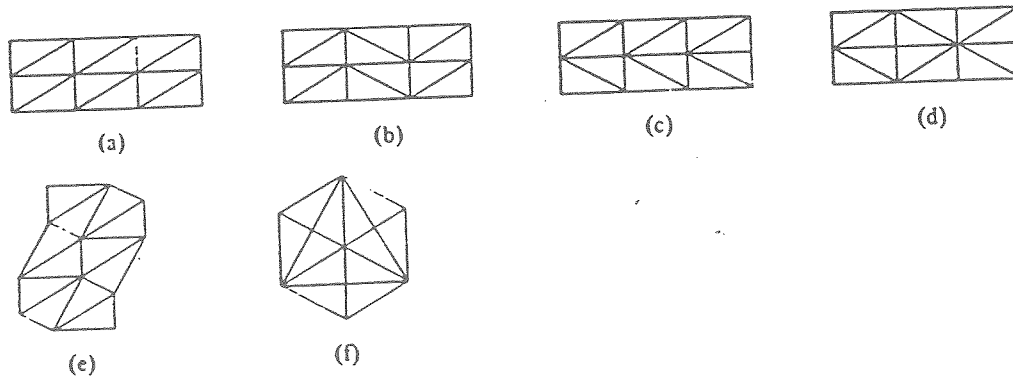
Figure 12. Six triangular tessellations.
