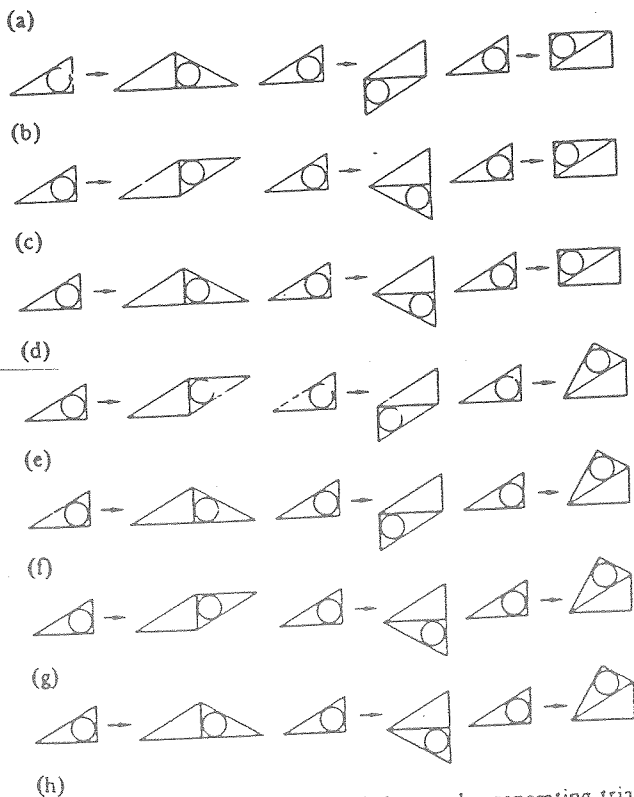
Figure 11. A shape grammar and shape rules generating triangular tessellations.
