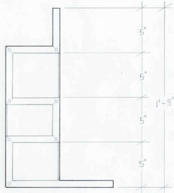
LEFT ELEVATION
